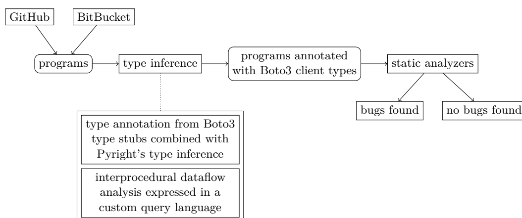
■ Figure 1 High-level overview of CodeGuru
