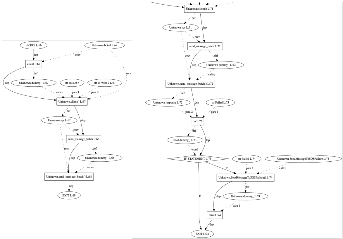
■ Figure 13 Complete MU Graph (left) for the non-compliant code and partial MU Graph (right) for the compliant code of Figures 14 and 15, respectively
