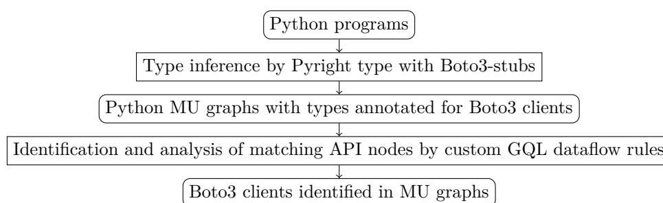
■ Figure 10 Layered type inference
