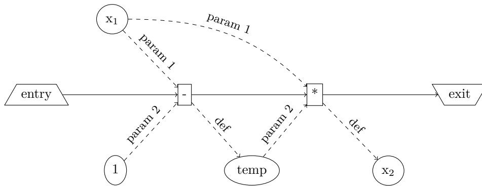
■ Figure 4 The MU-graph representation of x *= x - 1 . Entry and exit nodes are trapezoidal; action nodes are rectangular; data nodes are elliptic. Control edges are solid; data edges are dashed.
