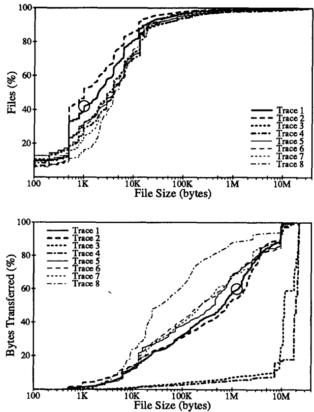
Figure 2. File size. Dynamic distribution of file sizes, measured when files were closed. The top graph is a cumulative distribution weighted by number of files, and the bottom graph is weighted by the number of bytes transferred to or from the file. For example, the circles indicate that for Trace 1 42% of all accesses were to files less than one Kbyte long, but that during the same trace 40% of all bytes were transferred to or from files of at least one Mbyte in size.
