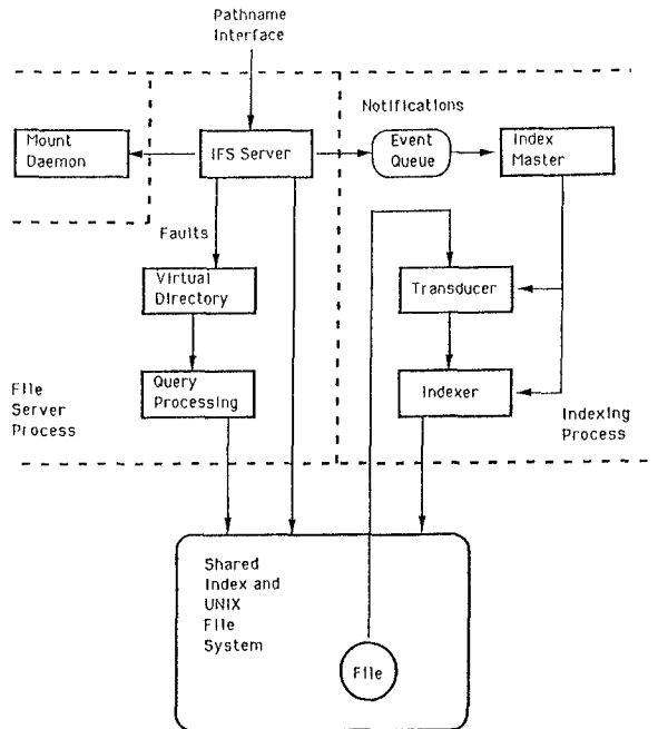
Figure 2: SFS Block Diagram
