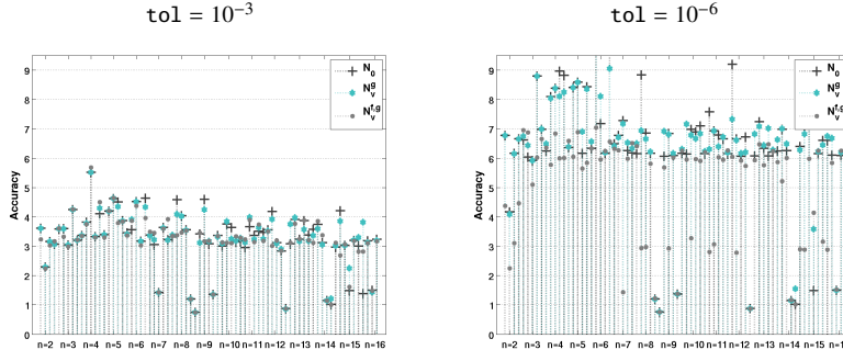
Fig. 3 Accuracy at termination for noise forms N_0 , N_v^{f,g} , and N_v^g .
