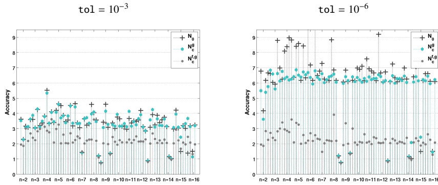
Fig. 2 Accuracy at termination for noise forms N_0 , N_c^{f,g} , and N_c^g .
