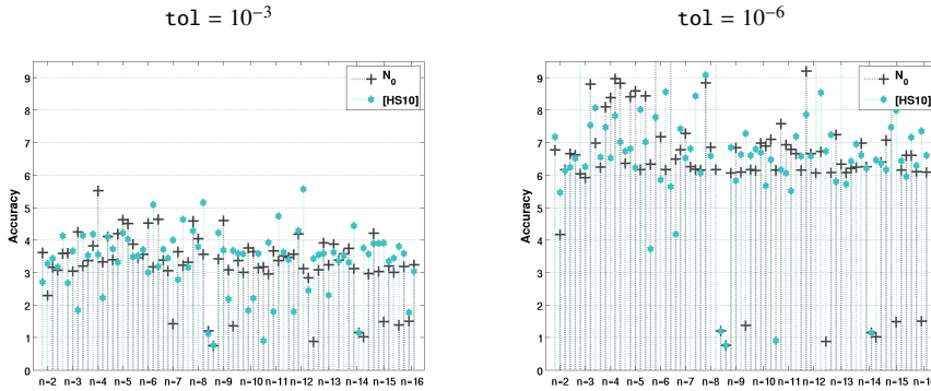
Fig. 1 Accuracy at termination for Algorithms 4 and [HS10].
