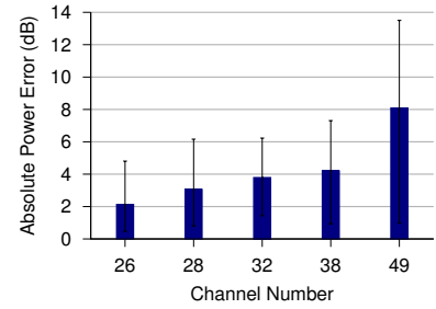
Figure 7: Median error in measuring the power of TV channels by Snoopy. Error bars show 10th and 90th quartile error.
