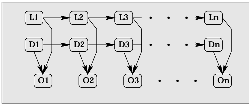
Figure 26. A Simple Dynamic Probabilistic Network with Two Independent State Variables: Robot Location ( L_i ) and Camera Direction ( S_i ).
