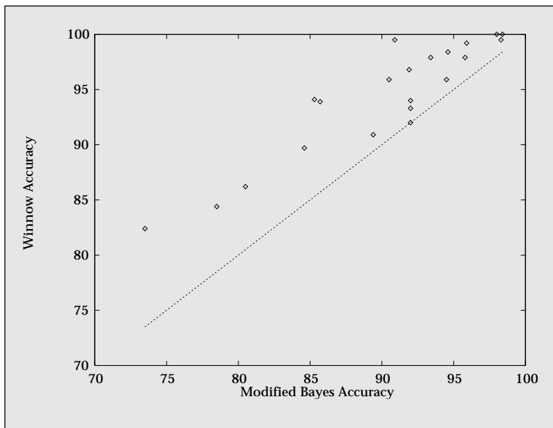
Figure 10. Comparison of the Percentage of Correct Classifications for a Modified Bayesian Method and WINNOW for 21 Sets of Frequently Confused Words.
