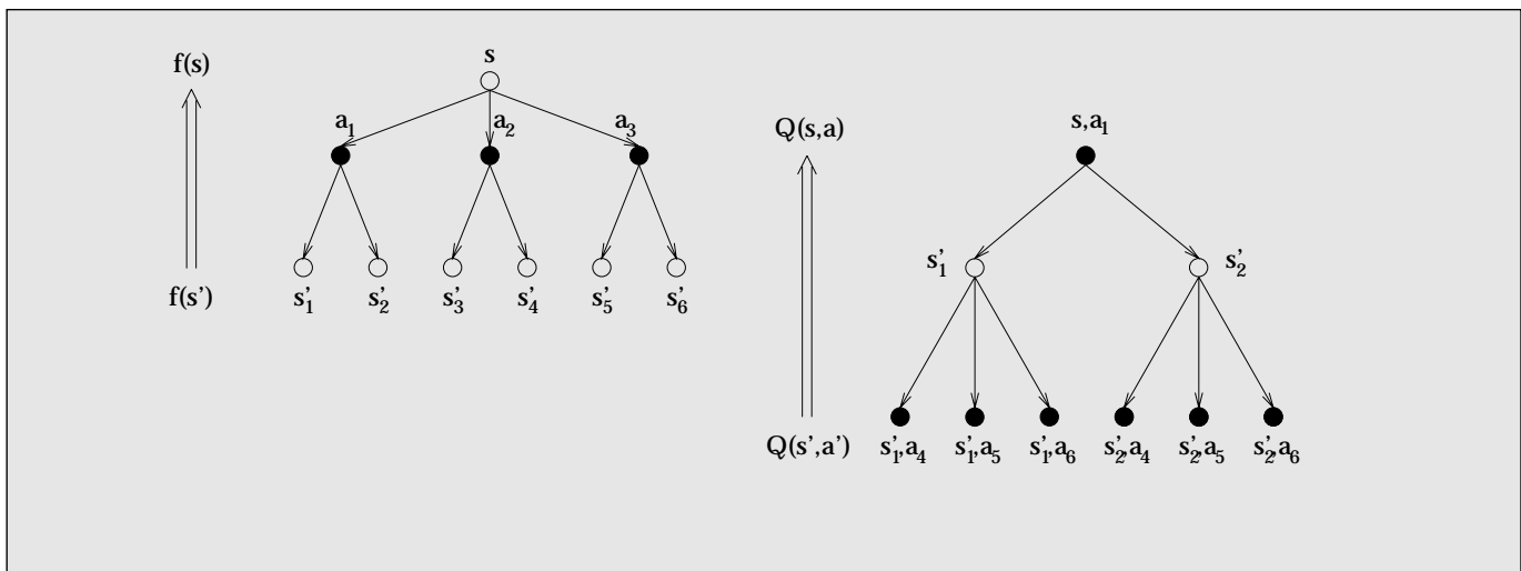
Figure 17. A Comparison of the Value Function f and the Q Function.
