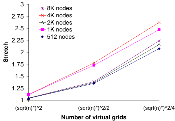
Fig. 9. Varying the number of virtual grids. \sqrt{n}^* represents the smallest power of 2 number that is greater than or equal to \sqrt{n} , where n is the number of nodes, i.e. \sqrt{n}^* = 2^{\lceil \log_2 \sqrt{n} \rceil} .
