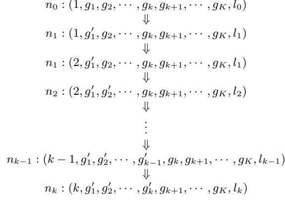
Fig. 8. An execution in T_1^s .
