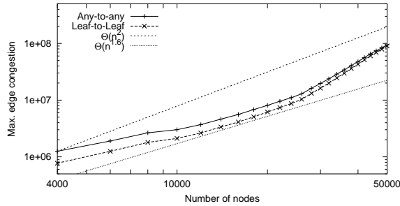
(a) Any-2-any and Leaf-2-leaf communication
