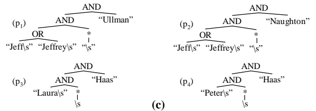
Figure 7: (a) A set of patterns p_1 - p_4 and a document d , (b) an inverted index over p_1 - p_4 , and (c) parse trees for p_1 - p_4 .
