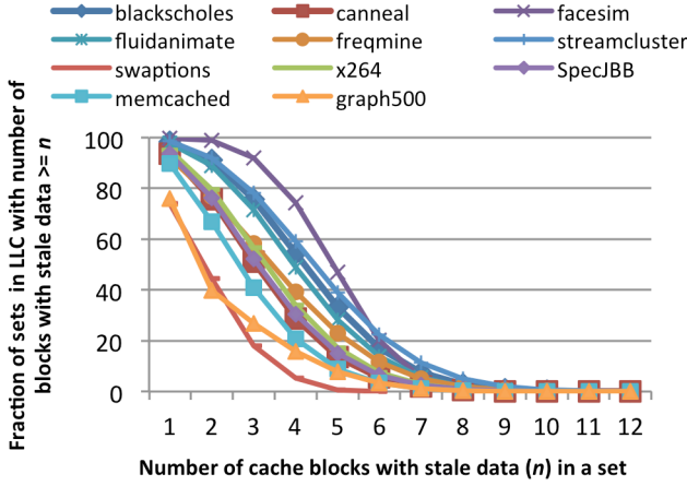
Figure 2. Distribution of stale blocks across sets.
