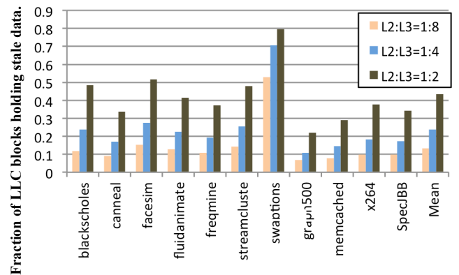
Figure 1. Portion of valid blocks with stale data.
