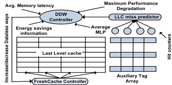
Figure 4. Hardware Control for Dynamic Dataless Ways (DDW). Additions are shaded.
