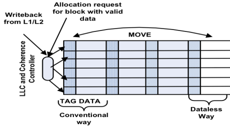
Figure 3. LLC controller with LLC having dataless ways.
