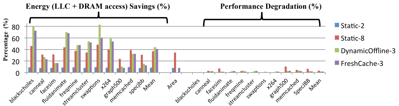
Figure 6. Energy savings and performance degradation for dynamic dataless ways under hardware control.
