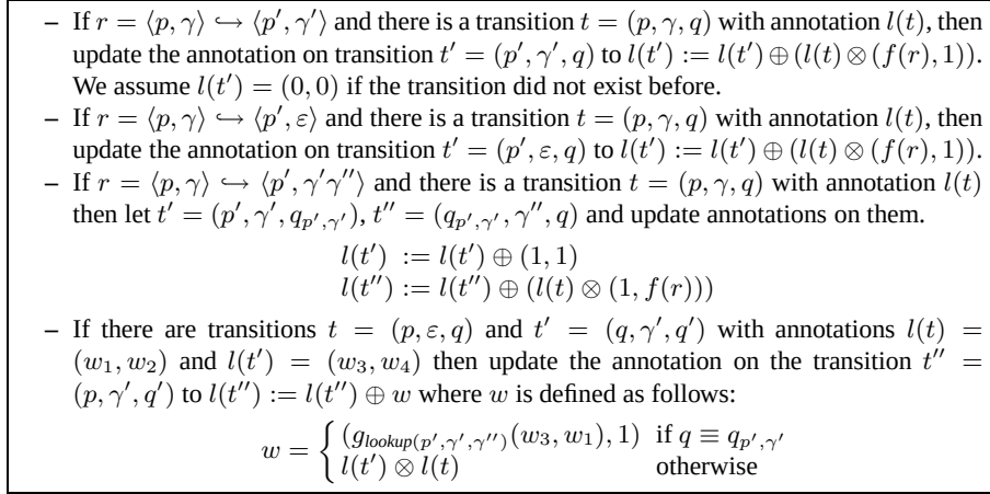
Fig. 3. Saturation rule for constructing \mathcal{A}_{post*} from \mathcal{A} .
