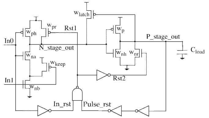
Fig. 7. Delayed-reset NAND2.
