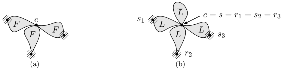
Figure 3: Connected component C' that might remain after removing a vertex cover S of G from G' , centered around a vertex c that has degree 3 in G and does not belong to S . (a) Naive construction. (b) Final construction.
