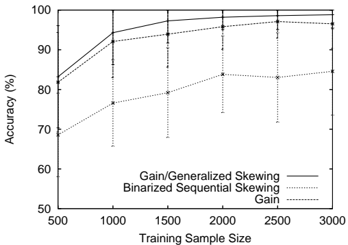
Figure 8. Random Nominal Targets, 30-v examples
