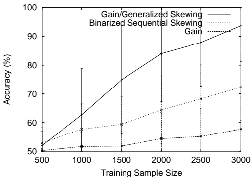
Figure 9. Hard Nominal Targets, 30-v examples
