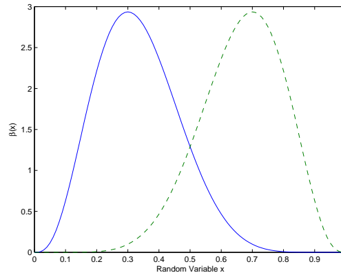
Figure 2. Beta distributions with a = 4 and b = 8 (solid line) and with a = 8 and b = 4 (dashed line). Larger values of a and b result in a higher peak and stronger skew.
