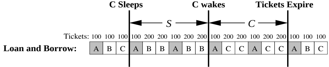
Figure 5.4: Stride-Scheduling with Loan & Borrow Extension. Three jobs with equal ticket allocations are competing for resources. Job A desires a constant service rate, job B is compute-intensive and willing to borrow tickets, and job C is an interactive job. Job C temporarily exits the system, and sleeps for an interval S ; in the time-interval C , job C catches up for the time it missed. All jobs receive their proportional-share of 6 allocations over the entire interval of 18 time-units; however, only this policy also supports jobs with precise allocation requirements; job A is always scheduled at least 1 out of every 3 time units regardless of the activity of other jobs.
