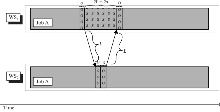
Figure 6.10: Cost with Network Latency when Processes are Coordinated and Spin-Wait. To help derive L_{Block} , this figure illustrates the cost of a request-reply for the sending and receiving processes when processes are coordinated and spin while waiting for communication to complete.
