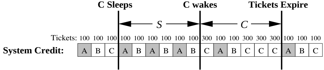
Figure 5.3: Stride-Scheduling with System Credit Extension. Three jobs with equal ticket allocations are competing for resources. Jobs A and B are compute-intensive and do not relinquish the processor; job C is an interactive job. Job C temporarily exits the system, and sleeps for an interval S ; in the time-interval C , job C catches up for the time it missed. All jobs receive their proportional-share of 6 allocations over the entire interval of 18 time-units
