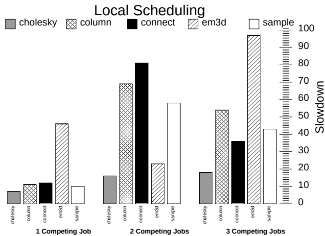
Figure 3.2: Simulated Performance of Local Scheduling versus Coscheduling. One real parallel application and one to three simulated parallel jobs are scheduled in a round-robin fashion with a 100ms time quantum on a 64-node CM-5. Slowdown is the ratio of the measured locally-scheduled execution time to the ideal coscheduled time.
