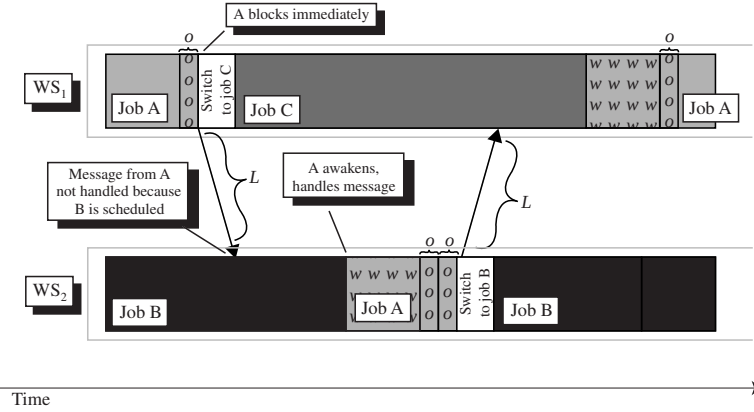
Figure 6.9: Cost with Network Latency when Processes are Uncoordinated and Block. To help derive L_{Block} , this figure illustrates the cost of a request-reply when processes are scheduled independently and block immediately rather than spin-wait for communication to complete.
