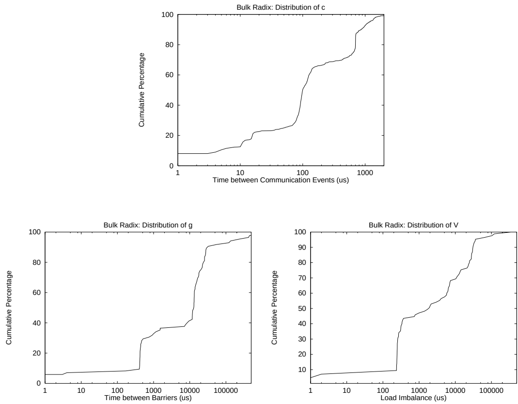
Figure 9.5: Communication Characteristics of Radix. The graphs show the distribution of the time between communication events ( c ), barriers ( g ), and load-imbalance ( V ) for Bulk Radix Sort. The measurements were taken for one job of 16 processes running on a dedicated system. The data shows that there is approximately 100\mu\text{s} of computation between 70% of the communication operations. Radix performs only about 80 barriers in its lifetime.
