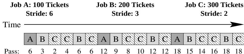
Figure 5.2: Basic Stride Scheduling. Three jobs ( A , B , and C ) with different ticket allocations are running on a single workstation. Each job has a stride and a pass associated with it. The stride of a job is inversely proportional to the number of tickets in the job. At each scheduling interval, the job with the minimum pass is scheduled and its pass is incremented by its stride .
