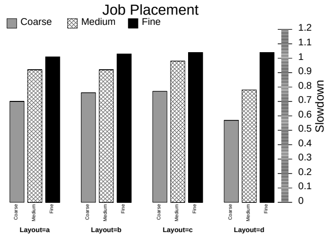
Figure 10.13: Sensitivity to Job Placement. Three or four jobs, A , B , C , and, optionally, D are placed across 16 workstations. The figures designate how the processes would be scheduled over time with explicit coscheduling. For each of the four layouts, we investigate three workloads: coarse, medium, and fine. The coarse-grain workload consists of applications synchronizing every g = 100\text{ms} with V = 200\text{ms} ; the medium-grain workload contains applications synchronizing every g = 10\text{ms} with V = 5\text{ms} ; finally, the fine-grain workload contains applications synchronizing every g = 100\mu\text{s} with V = 0 . All workloads read in a NEWS pattern with c = 8\mu\text{s} of intervening computation.
