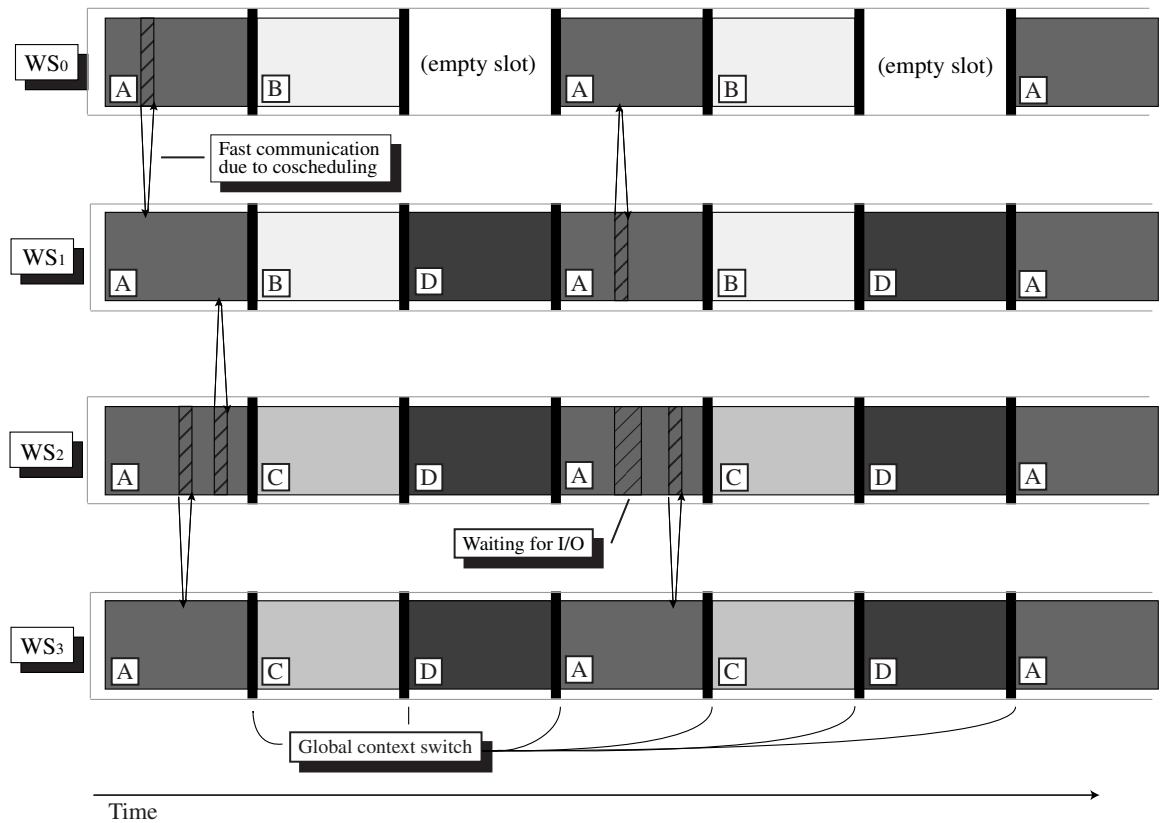
Figure 3.3: Explicit Coscheduling Matrix. Four parallel jobs (A, B, C, and D) are allocated to four workstations. With explicit coscheduling, or gang scheduling, the system guarantees that communicating processes are scheduled simultaneously across workstations. As a result, when network latency and load-imbalance are low, processes can spin-wait for message replies without wasting significant amounts of CPU. However, to scheduled processes under such constraints, empty slots may exist in the global schedule where no process can run simultaneously with the other processes in its job. Further, processes must spin-wait when they perform I/O, not allowing another process to perform useful computation.
