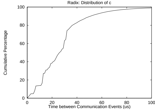
Figure 9.7: Communication Characteristics of Radix:Small. Because this version of Radix Sort performs very few barriers, the graphs for g and V are not shown. The graph shows that there is only 30\mu s of computation (including the overhead of collecting the tracing information) between 75% of communication operations.
