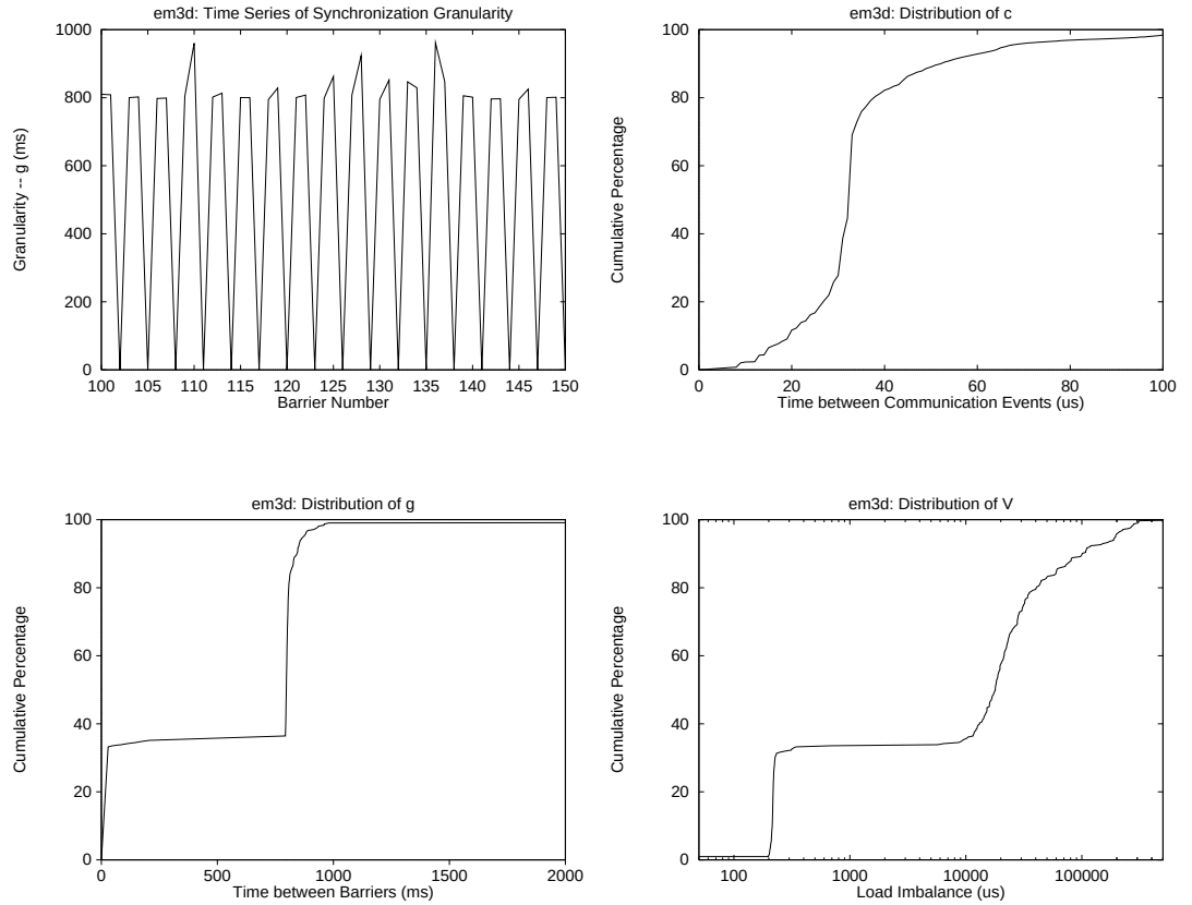
Figure 9.6: Communication Characteristics of EM3D. The first graph shows the regular nature of EM3D, in which e -nodes and h -nodes are calculated in turn for a number of time-steps. The main loop of the application contains three barriers: one at the beginning of the time-step, one after performing the calculations for e -nodes, and one after the calculations for h -nodes. Thus, the average time for each e -node or h -node step across all processes is about 800ms. The remaining graphs show the distribution of the time between communication events ( c ), barriers ( g ), and load-imbalance ( V ). The barriers after the e -node and h -node calculations have between V = 10\text{ms} and V = 300\text{ms} worth of load-imbalance.
