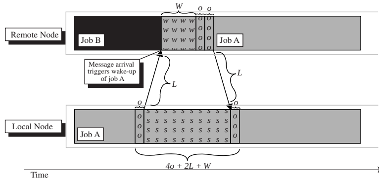
Figure 6.2: Time for Request-Response Message with Triggering of Remote Process. The diagram illustrates T_{Trigger}^R , the amount of time a local process must wait for a reply if the request message triggers the scheduling of the remote destination process. In this case, the local process must spin-wait the additional time, W , while waiting for the remote process to be scheduled by its local operating system scheduler.
