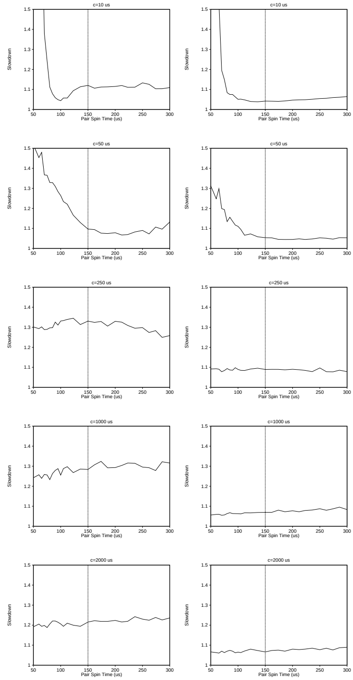
Figure 8.9: Closeups of Sensitivity to Conditional Spin Amount ( W = 50\mu s ).
