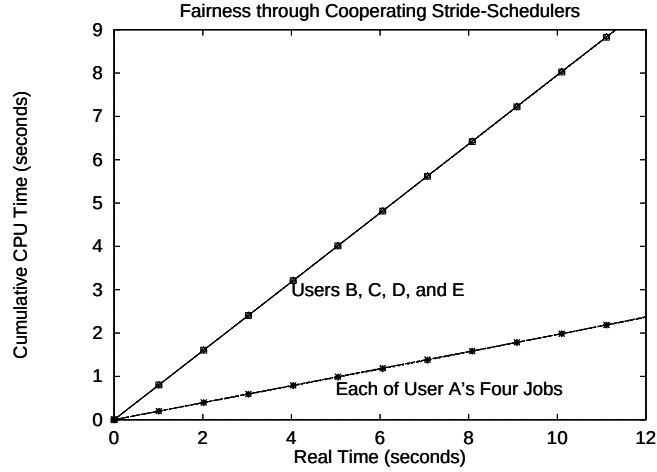
Figure 5.7: Measured Fairness with Ticket Server and Stride Scheduler. Five competing users are running compute-bound sequential jobs on a cluster of four workstations. User A is running one job on each of the four workstations, while the other users are running only one job each. The parallel ticket server informs the stride scheduler running on each workstation of the number of tickets user A has allocated across the cluster, so that user A receives only 1/5 of each workstation, as desired.
