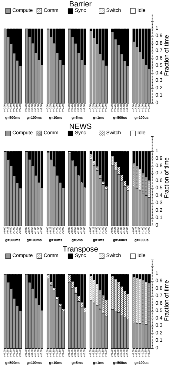
Figure 7.2: Characteristics of Bulk-Synchronous Benchmarks. The three graphs show the breakdown of execution time for the three communication patterns. Along the x axis, the computation granularity, g , and the load-imbalance, V , are varied. Within a group of six bars, each job has the same computation granularity. Groups on the left are relatively coarse-grained; groups on the right are more fine-grained. Within each group, the load-imbalance is increased as a function of the granularity: from V = 0 to V = 2 \cdot g . The fraction of execution time is divided into three components (computing, communicating, and synchronizing). Note that the Barrier program performs no communication. This data assumes a network latency of 10\mu s .
