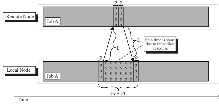
Figure 6.1: Time for Request-Response Message with Remote Process Scheduled. The diagram illustrates T_{Sched}^R , the amount of time a local process must wait for a reply if the remote destination process is scheduled when the request message arrives. If the remote destination process is already scheduled, then it immediately handles the request and promptly returns the reply to the waiting process.
