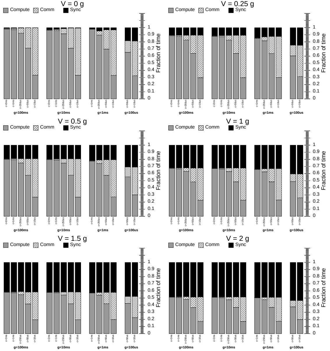
Figure 7.4: Characteristics of Continuous-Communication Benchmarks. The six graphs show the breakdown of execution time for r NEWS communication pattern as the load-imbalance, V , is varied. Along the x axis, the average time between barriers, g , and time between read operations, c , is varied. Groups of bars on the left are relatively coarse-grained; groups on the right are more fine-grained. The fraction of execution time is divided into three components (computing, communicating, and synchronizing). This data assumes a network latency of 10\mu s .
