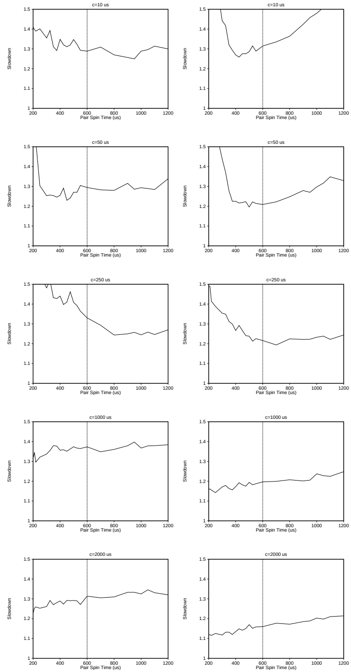
Figure 8.10: Closeups of Sensitivity to Conditional Spin Amount ( W = 200\mu s ).
