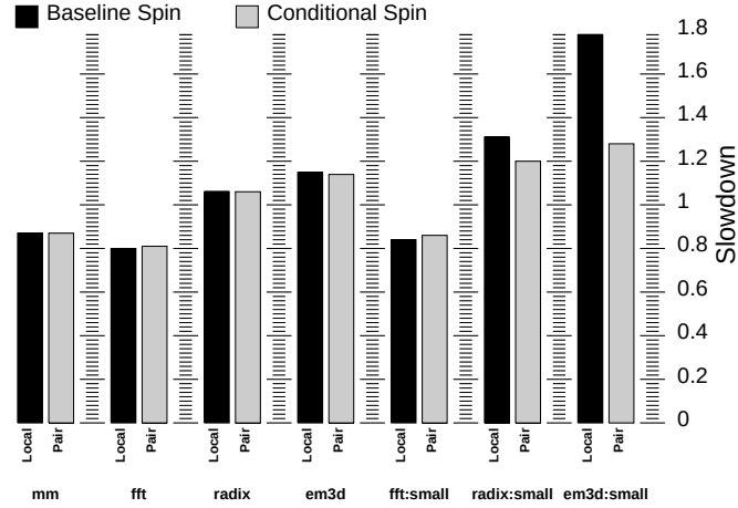
Figure 10.9: Performance of Real Split-C Applications. Three copies of each Split-C application are run on 16 workstations. The first four applications use bulk messages, while the last three use small messages. mm is matrix multiply; fft is a fast Fourier transform; radix is a radix sort; em3d models the propagation of electro-magnetic waves in three dimensions.
