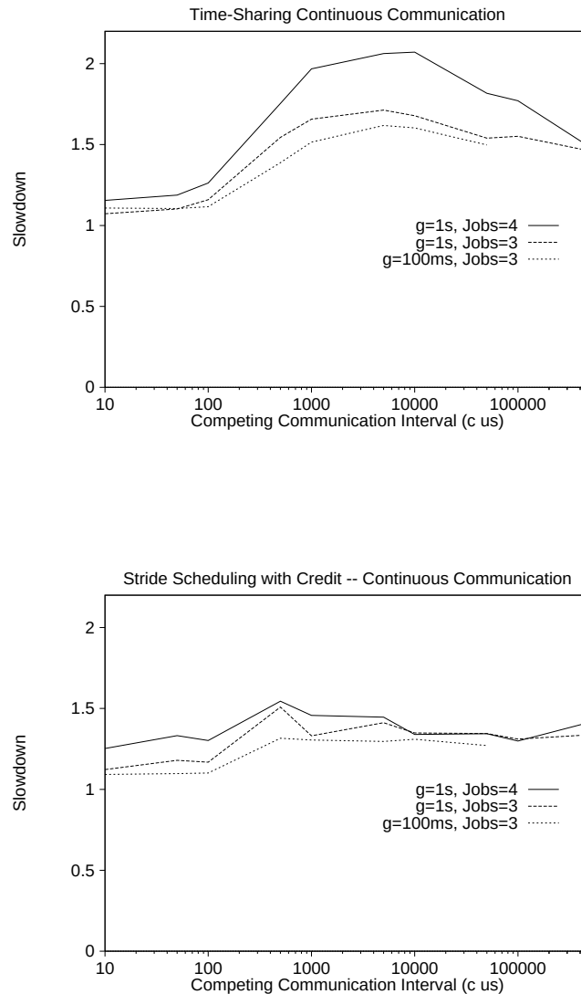
Figure 10.6: Fairness with Continuous-Communication Programs. One measured job and two or three competing background jobs are allocated to 16 workstations. Only the slowdown of the one job is measured; the background jobs run continuously during the experiment. We evaluate continuous-communication workloads where barriers are rarely performed. In each workload, the values of g are identical for all jobs (either g = 100\text{ms} or g = 1\text{s} ), there is no load-imbalance, and processes read from remote processes in a Random pattern. The examined job has the interval between reads set at c = 50\mu\text{s} , while c is varied for the two or three background jobs. The first graph uses the default Solaris Time-Sharing scheduler on each workstation; the second graph uses our implementation of the Stride Scheduler with System Credit.
