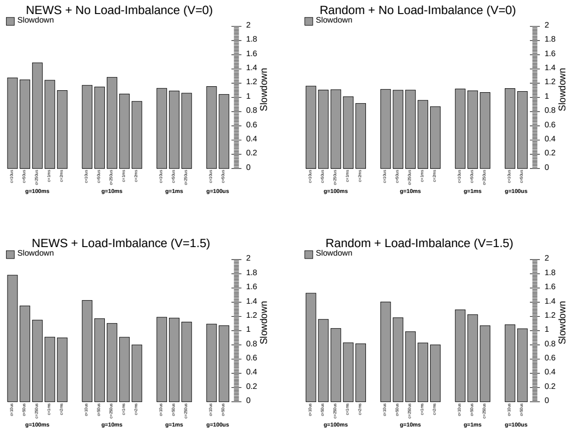
Figure 10.4: Performance of Continuous-Communication Programs with Request-Response Messages. The workload consists of three jobs running on 16 workstations. Each application communicates with request-response (read) messages in either the NEWS or Random pattern. The time between barriers is varied between g = 100\mu s and g = 100ms and the time between reads is also varied between c = 10\mu s and c < g . The applications in the first set of graphs have no load-imbalance ( V = 0 ); in the second set of graphs, the load-imbalance is V = 1.5g .
