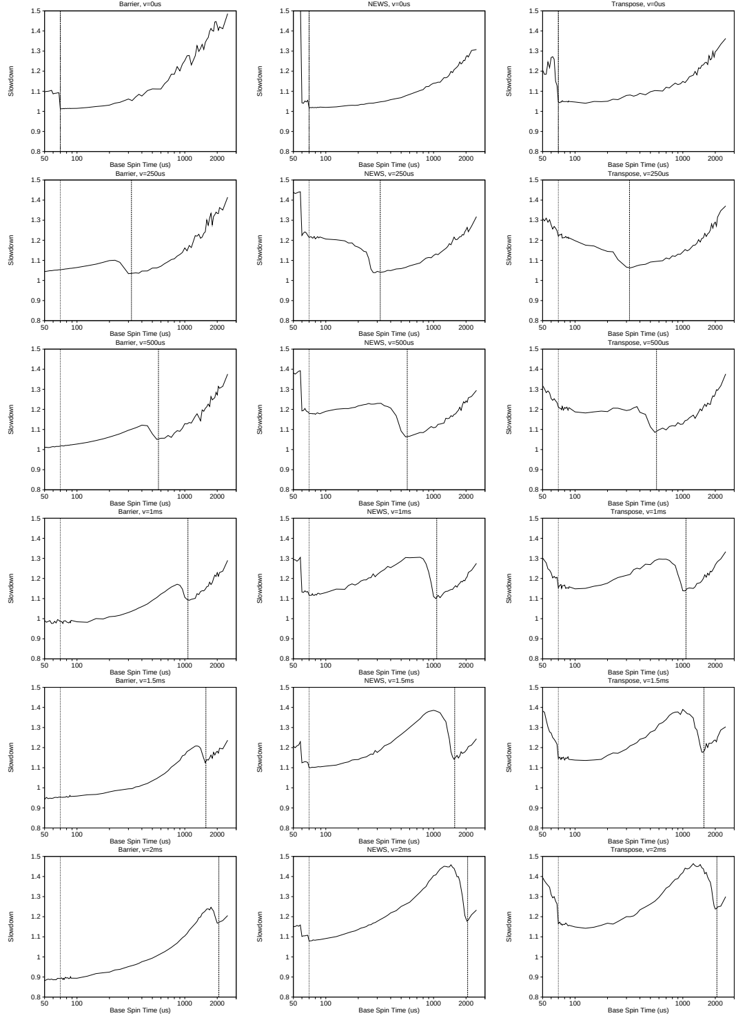
Figure 8.12: Sensitivity to Baseline Spin for Bulk-Synchronous Programs with Load-Imbalance ( W = 50\mu s ).
