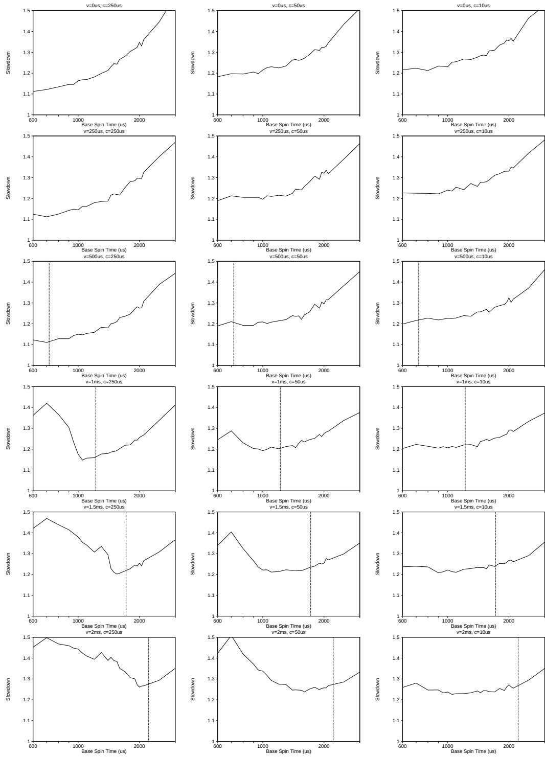
Figure 8.15: Sensitivity to Baseline Spin for Bulk-Synchronous Programs with Load-Imbalance ( W = 200\mu s ).
