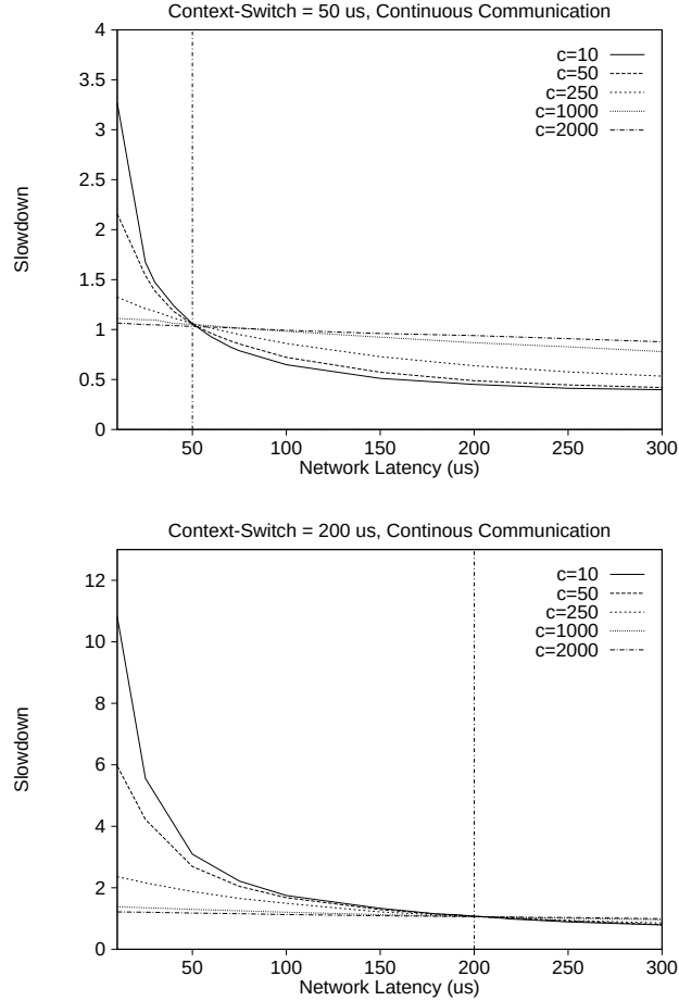
Figure 8.1: Impact of Latency and Context-Switch Time on Continuous-Communication Workloads. Each workload consists of three competing jobs each containing 32 processes time-shared on a total of 32 workstations. Each of the three jobs follows the continuous communication model. The time between barriers, g , is 100ms, and there is no load-imbalance ( V = 0 ). Each process communicates with its four nearest neighbors in a regular NEWS pattern. Each line in the graph designates a different communication granularity; the average time between reads, c , is set to 10, 50, 250, 1000, and 2000 \mu s. The metric along the y-axis is the slowdown of the workload when scheduled independently with immediate blocking versus explicit coscheduling with spin-waiting. In each graph, network latency, L , is increased from 10 \mu s to 300 \mu s along the x-axis. The vertical lines designate the point where L = W . Note the change in scales in the y-axes across the two graphs. Context-switch time is changed in the two graphs from W = 50\mu s to W = 200\mu s.
