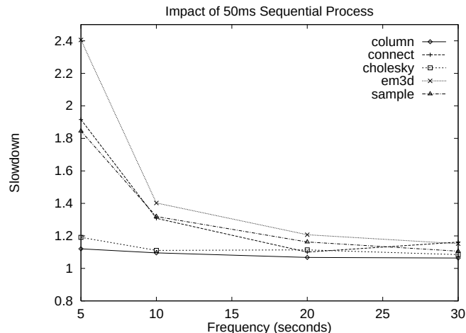
Figure 3.4: Impact of Interactive Processes on Parallel Jobs. Each of the parallel applications is periodically interrupted at an random time on one of 64 nodes of the CM-5. The 50ms interruption simulates a short-lived process arriving on one of the workstations in the cluster. During this interruption, messages arriving for the parallel program are buffered and the sending process must spin-wait for a longer interval. Along the x-axis, the inter-arrival time of the interrupting processes on each workstation is varied between 5 and 30 seconds. The y-axis is the slowdown of the process with interruptions versus that in a dedicated environment.
