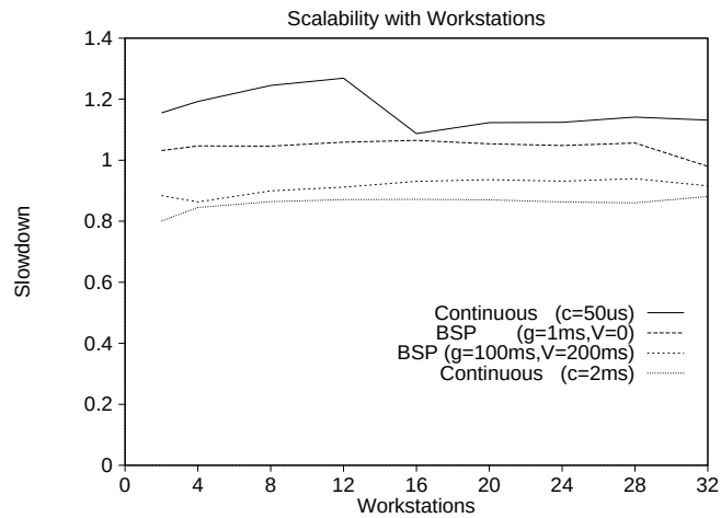
Figure 10.12: Workstation Scalability. Three competing jobs are allocated to an increasing number of workstations. We evaluate two continuous-communication and two bulk-synchronous workloads. In both continuous-communication workloads, barriers are rarely performed (i.e., g = 100ms ), there is no load-imbalance, and processes read from remote processes in the Random pattern. In the fine-grain workload, processes communicate every c = 50\mu s ; in the medium-grain workload, processes communicate every c = 2ms . The bulk-synchronous workloads read from remote processors in the NEWS pattern. The first bulk-synchronous workload represents medium-grain applications ( g = 1ms ) with no load-imbalance ( V = 0 ); the second bulk-synchronous workload represents coarse-grain applications ( g = 100ms ) with a large amount of load-imbalance ( V = 200ms ).
