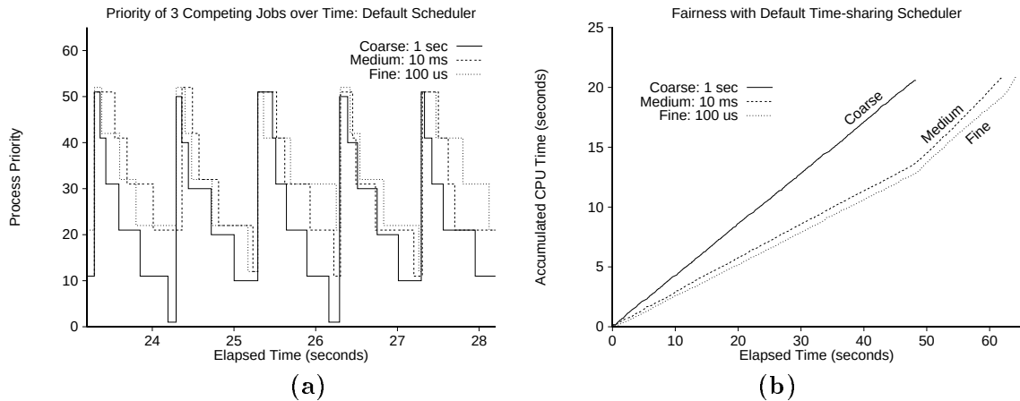
Figure 5.1: Measured Fairness with Solaris Time-Sharing Scheduler. Three bulk-synchronous jobs communicating with the NEWS pattern and no load-imbalance are time-shared on 16 workstations. To capture this data, we ran the three parallel jobs with implicit coscheduling in our system, while recording all changes to the priority of each process on a single workstation.
