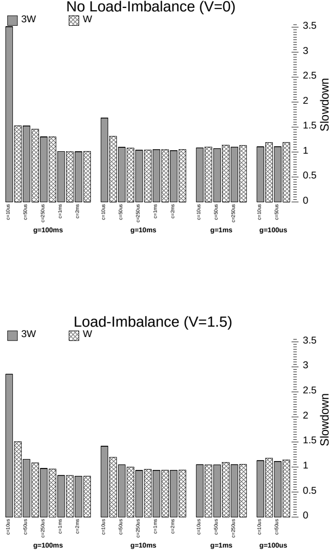
Figure 10.7: Performance of Continuous-Communication Programs with One-Way Requests. Each application communicates with one-way request (store) messages in the NEWS pattern. The first bar in each set shows the slowdown when processes perform conditional spinning with S_{Cond}^O = 3W ; the second bar in each set assumes S_{Cond}^O = W . The workload consists of three jobs running on 16 workstations. The time between barriers is varied between g = 100\mu s and g = 100ms and the time between reads is also varied between c = 10\mu s and c < g . The applications in the first graph have no load-imbalance ( V = 0 ); in the second graph, the load-imbalance is V = 1.5g .
