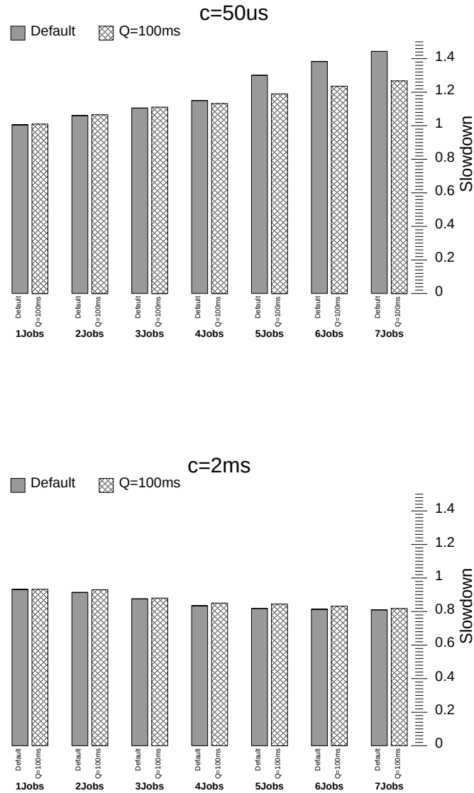
Figure 10.11: Job Scalability with Continuous-Communication Programs. The number of jobs in the system is increased from one to seven. We investigate only the case where processes are allocated identically across jobs. We compare the performance of the Default Solaris Time-sharing scheduler to one modified to use Q=100ms time-slices for all priorities. In both workloads, barriers are rarely performed (i.e., g = 100ms ), there is no load-imbalance, and processes read from remote processes in the Random pattern. In the fine-grain workload on the left, processes communicate every c = 50\mu s ; in the medium-grain workload on the right, processes communicate every c = 2ms .
