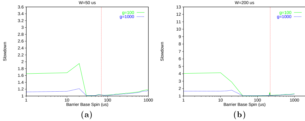
Figure 8.6: Sensitivity to Barrier Baseline Spin for Bulk-Synchronous Programs. The environment and workloads are identical to that in the previous figure. Along the x -axis, the baseline spin for barriers is varied while the read spin time is kept constant at S_{Base}^R . The vertical line in each graph designates the desired barrier baseline spin, S_{Base}^B = 2L + W . In Figure a, the context-switch time is set to W = 50\mu s ; in Figure b, W = 200\mu s .
