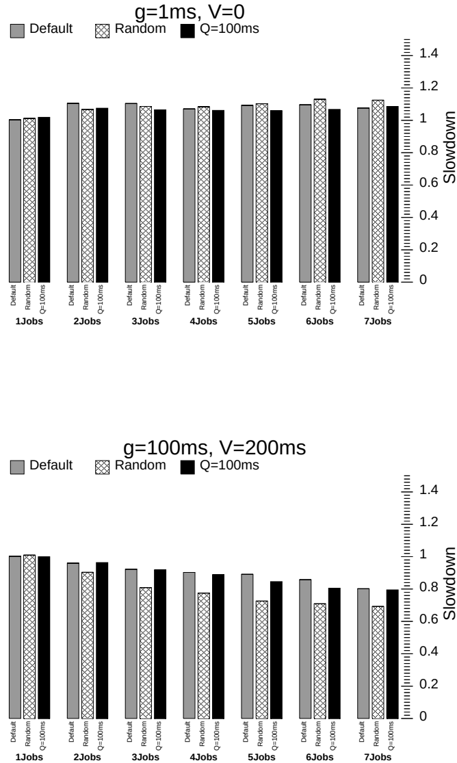
Figure 10.10: Job Scalability with Bulk-Synchronous Programs. The number of jobs in the system is increased from one to seven, each running on 16 workstations. Within each graph we investigate three slight variations on the placement of jobs and on the local operating system scheduler. In the Default case, processes are placed with an identical layout across nodes. In the Random case, processes are randomly placed on different nodes. Finally, with Q=100ms , processes are placed identically across workstations as in the Default case, but the local scheduler is modified to use Q = 100\text{ms} time-slices at all priority levels. Each workload reads from remote processors in the NEWS pattern. The first bulk-synchronous workload represents medium-grain applications ( g = 1\text{ms} ) with no load-imbalance ( V = 0 ); the second bulk-synchronous workload represents coarse-grain applications ( g = 100\text{ms} ) with a large amount of load-imbalance ( V = 200\text{ms} ).
