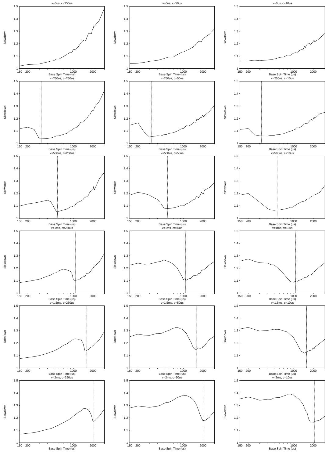
Figure 8.14: Sensitivity to Baseline Spin for Continuous-Communication Programs with Load-Imbalance ( W = 50\mu s ).
