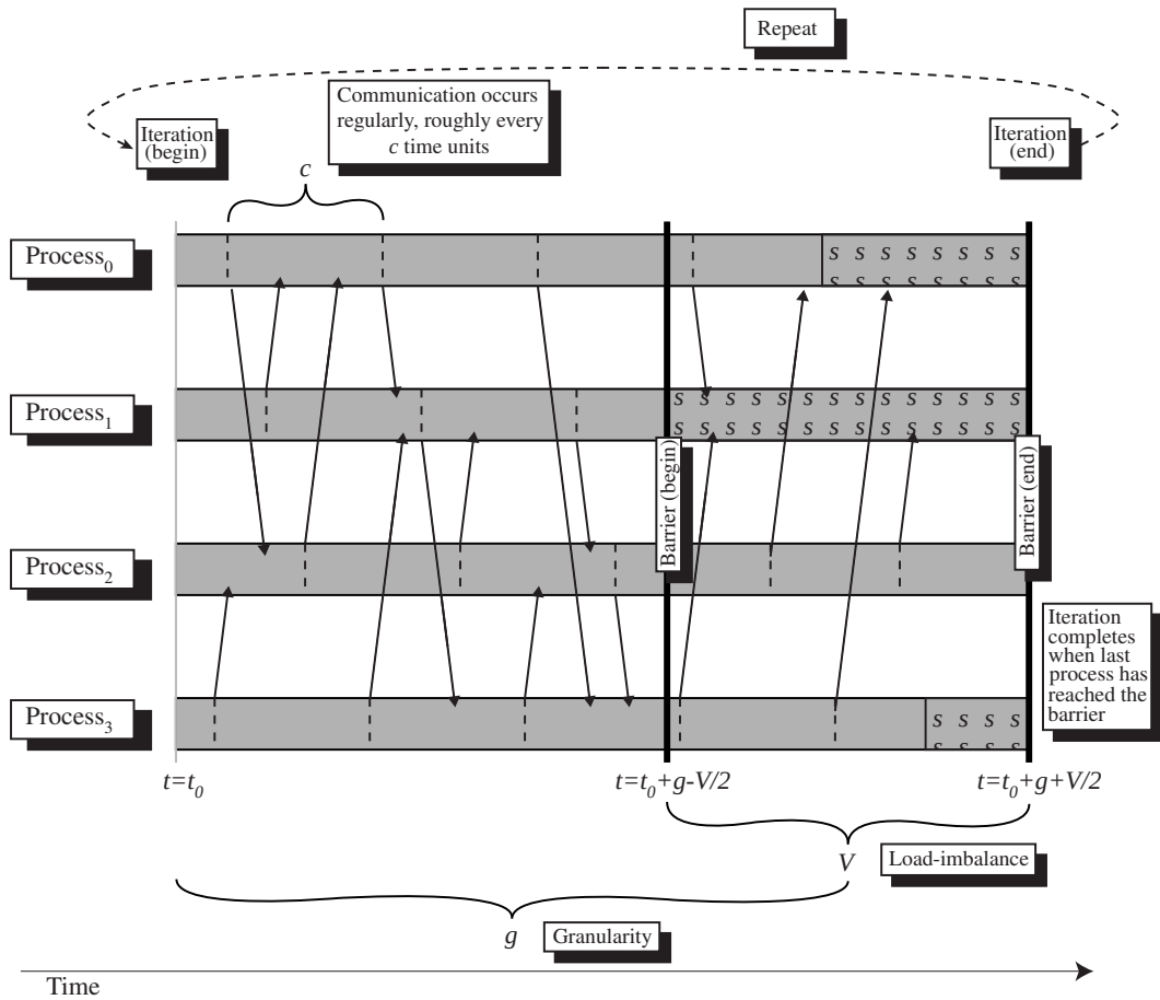
Figure 7.3: Model of Continuous-Communication Synthetic Parallel Applications. Each process continuously communicates with other cooperating processes running on other processors. The average time between communication requests for a given process is c time units. Each process also periodically performs a barrier; the mean time between barriers is g , chosen uniformly from the interval (g - V/2, g + V/2) .
