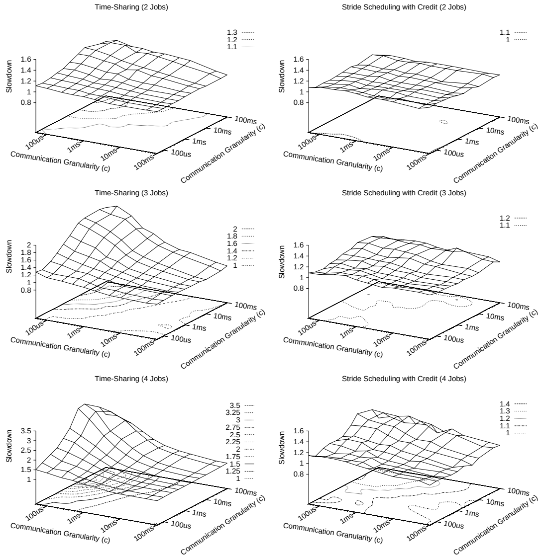
Figure 8.20: Fairness for Continuous-Communication Programs ( g = 100\text{ms} ). Jobs continuously communicating with the NEWS pattern and no load-imbalance are time-shared on 32 workstations. The processes of each job are randomly placed across workstations. Along the x-axis, the time between reads for the job under evaluation is varied between 50\mu\text{s} and 100\text{ms} . Along the y-axis, the time between reads is varied for a continuously running competing job. The metric along the z-axis is the slowdown of the evaluated job with implicit coscheduling and the full two-phase waiting algorithm (ideal baseline and pairwise spin times) versus explicit coscheduling with spin-waiting. Note the change in scale as the number of jobs is increased with the Solaris Time-Sharing scheduler.
