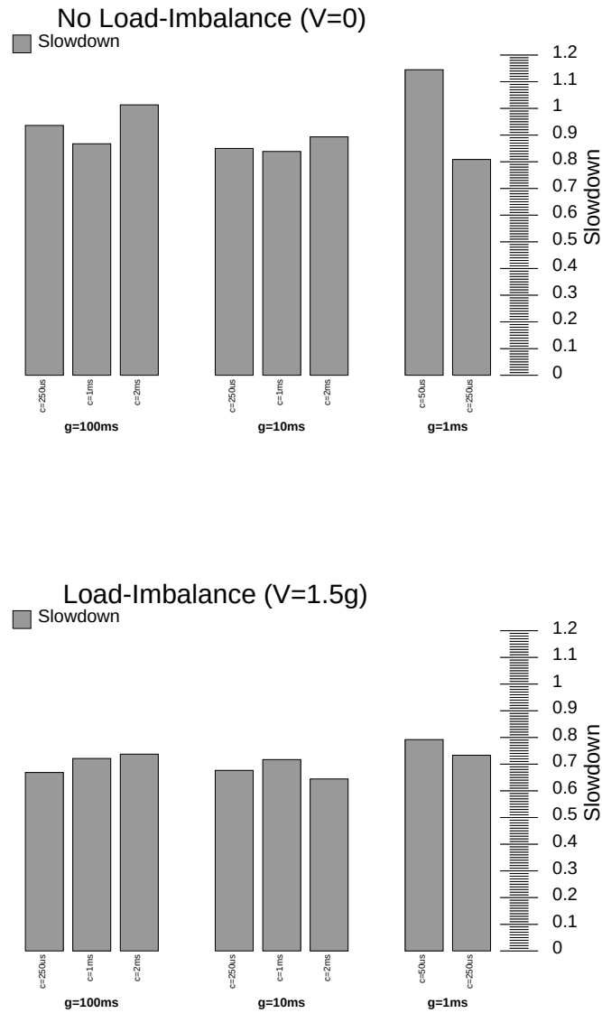
Figure 10.8: Performance of Continuous-Communication with Bulk Messages. Each application repeatedly requests 16KB messages (i.e., reads) from neighbors in the NEWS pattern. The workload consists of three jobs running on 16 workstations. Not as many workloads are shown as for the previous experiments: the time between barriers is varied between g = 1\text{ms} and g = 100\text{ms} and the time between reads is varied between c = 50\mu\text{s} or c = 250\mu\text{s} and c < g . The applications in the first graph have no load-imbalance ( V = 0 ); in the second graph, the load-imbalance is V = 1.5g .
