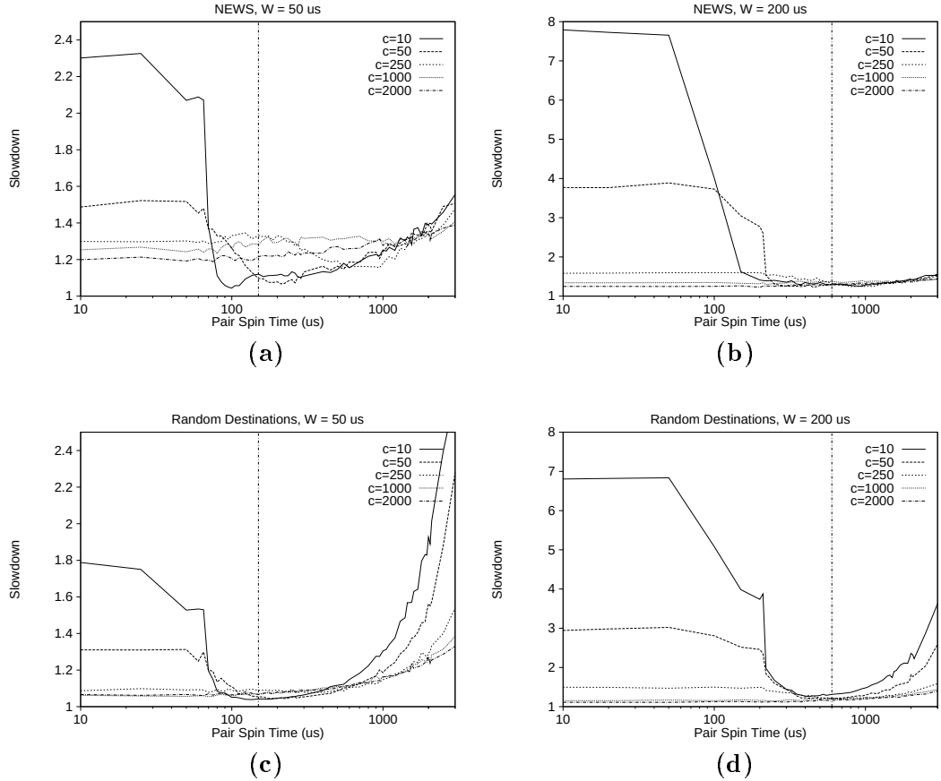
Figure 8.8: Sensitivity to Conditional Spin for Continuous-Communication Programs. The workload consists of three continuously communicating jobs on 32 workstations. The time between barriers is set to g = 100\text{ms} with no load-imbalance ( V = 0 ). Each line in the graphs designates a different communication granularity, c . The metric along the y-axis is the slowdown of the workload when implicitly coscheduled with two-phase waiting versus explicit coscheduling with spin-waiting. Along the x-axis, the pairwise spin time for both reads and barriers are changed simultaneously. The vertical line marks 3W , our chosen value of S_{Cond}^R . In Figures a and c, the context-switch cost is set to W = 50\mu\text{s} ; in Figures b and d, W = 200\mu\text{s} ; note the change in scale along the y-axis between the two sets. In the top two graphs, processes communicate in a repeated NEWS pattern; in the bottom two graphs, processes communicate with random destinations.
