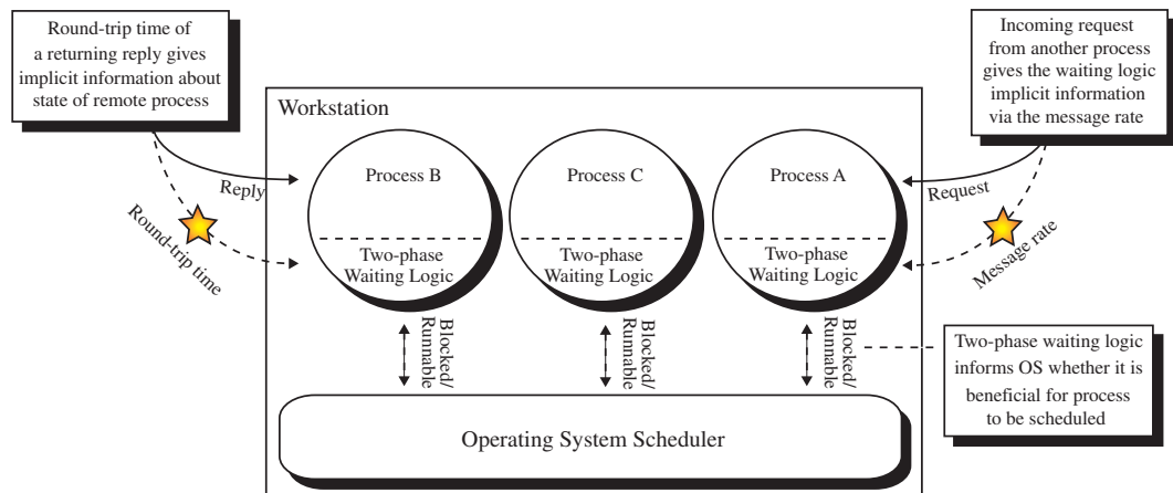
Figure 4.1: Transfer of Information in Implicit Coscheduling. Processes that are part of a communicating job receive implicit control information from the processes they are currently communicating with. This information is used as part of the two-phase waiting logic within each communicating process. From the round-trip time of returning reply message and from the arrival of incoming messages, the local process can infer whether the remote process is likely to be currently scheduled. The local process informs the operating system scheduler whether it is beneficial to be scheduled by either remaining runnable or by blocking until a message arrives.
