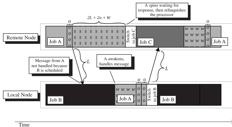
Figure 6.6: Cost of Incoming Request-Response Messages if Local Process Blocks. To help calculate T_{Cond}^R , the figure illustrates the cost to the pair of processes when the local process blocks while waiting for message arrivals.
