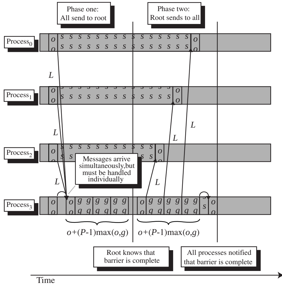
Figure 6.3: Time for All-to-all Synchronization with Processes Scheduled. The diagram shows T_{Sched}^B , the time for a barrier with no load-imbalance to complete if all participating processes are scheduled in a coordinated fashion. The diagram illustrates T_{Sched}^B from the perspective of the last process to be notified that the barrier has completed.
