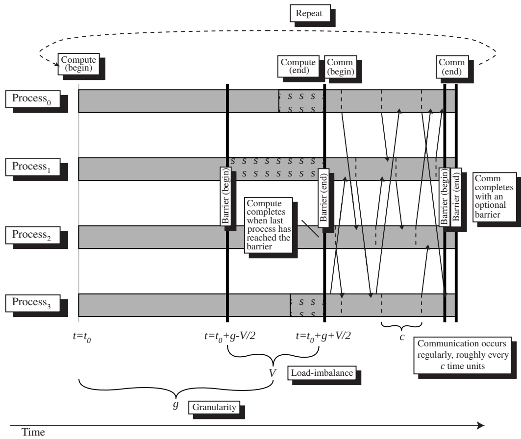
Figure 7.1: Model of Bulk-Synchronous Synthetic Parallel Applications. Each process of a parallel job executes on a separate processor and alternates between computation and communication phases. Processes compute for a mean time g before executing the opening barrier of the communication phase; the variation in computation across processes is uniformly distributed in the interval (0, V) . Within the communication phase, each process computes for a small time, c , between reads; the communication phase ends with a barrier.
