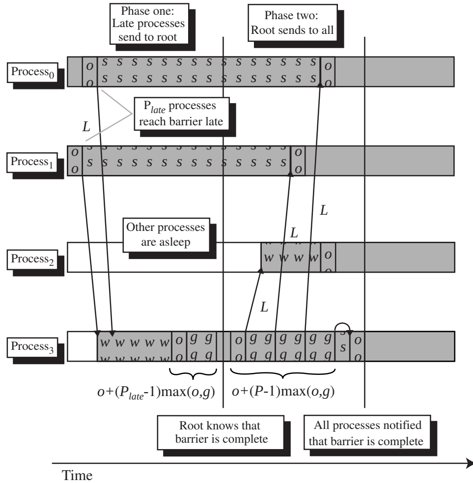
Figure 6.4: Time for All-to-all Synchronization with Triggering of Root Process. The diagram illustrates T_{Trigger}^B , the amount of time the last process notified must wait if the root process was not scheduled when the last set of P_{late} notification messages arrived.
