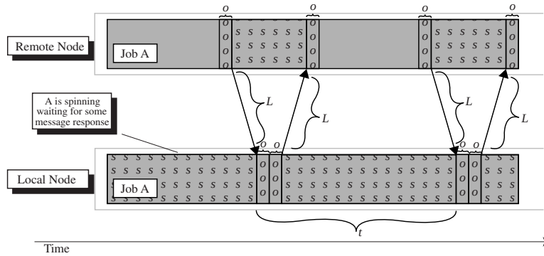
Figure 6.5: Cost of Incoming Request-Response Messages if Local Process Spin-Waits. To help calculate T_{Cond}^R , this figure illustrates the cost to the local (receiving) process and the remote (sending) process when the local process spin-waits between message arrivals. We assume a constant time t between message arrivals.
