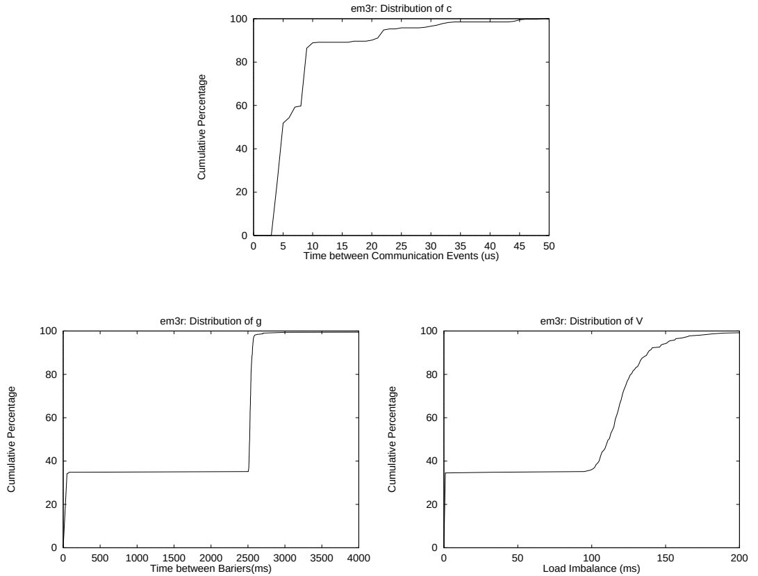
Figure 9.8: Communication Characteristics of EM3D:Small. The version of EM3D:Small proceeds in time-steps like EM3D shown in Figure 9.6; however, communication occurs much more frequently ( c \approx 10\mu s ) and the time-steps are significantly slower ( g \approx 2.5s ).
