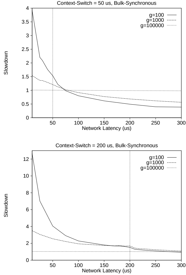
Figure 8.2: Impact of Latency and Context-Switch Time on Bulk-Synchronous Workloads. Each workload consists of three competing jobs consisting of 32 processes each time-shared on 32 workstations. Each of the three jobs follows the bulk-synchronous communication model. Each line designates a different synchronization granularity; the time between barriers, g , is set to 100\mu s , 1ms , and 100ms . There is no load-imbalance ( V = 0 ), and the time between reads to the four nearest-neighbors, is fixed at c = 8\mu s . The metric along the y-axis is the slowdown of the workload when scheduled independently with immediate blocking versus explicit coscheduling with spin waiting. Network latency, L , is increased from 10\mu s to 300\mu s along the x-axis. The vertical lines designate the point where L = W . Note the change in scales in the y-axes across the two graphs. Context-switch time is changed in the two graphs from W = 50\mu s to W = 200\mu s .
