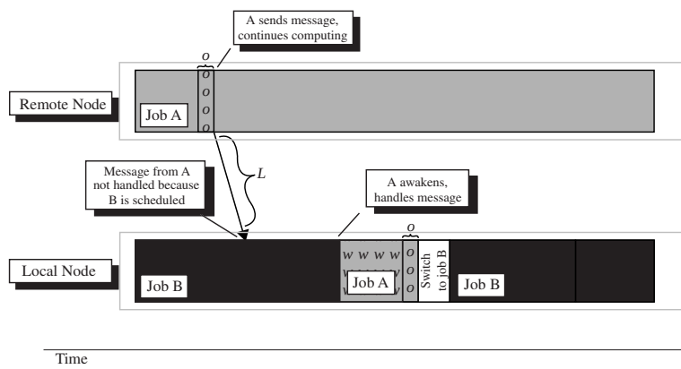
Figure 6.8: Cost of One-Way Requests if Local Process Blocks. To help calculate T_{Cond}^R , the figure illustrates the cost to the local process when it blocks while waiting for incoming messages.
