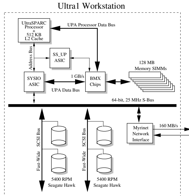
Figure 9.1: Internals of Ultra 1 Workstation. The figure depicts the internal architecture of an Ultra1 workstation. The Network Interface Card is connected to the S-Bus of each workstation.
