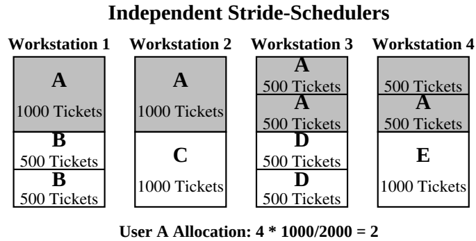
Figure 5.5: Fairness in Cluster with Independent Stride Schedulers. With independent proportional-share schedulers, users do not necessarily receive their expected share. In this example, users A, B, C, D, and E each have 1000 tickets in the base currency; in a cluster of four machines, each user should receive 4/5 of the time on one workstation. With the current placement of two users per workstation, if each scheduler independently calculates tickets then each user receives half of a workstation. Therefore, user A receives more resources by running on all of the workstations.
