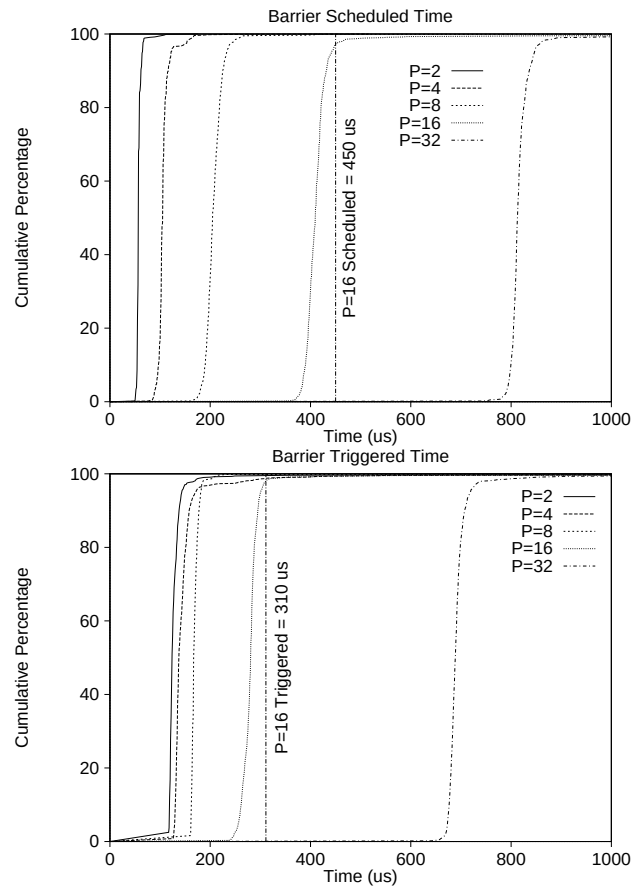
Figure 9.4: Microbenchmark Results for Linear Barrier Baseline Spin. The top graph shows the distribution of barrier completion times (from the perspective of the process notified last) if all participating processes are coordinated and send notification messages simultaneously to the root process. The bottom graph shows the distribution when all but one process arrive at the barrier early and block until the barrier is completed; when the last notification message arrives at the root process, it is scheduled and sends responses to all processes. The number of participating processes is increased from two to 32 in both sets of measurements.
