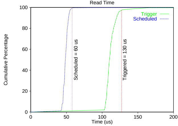
Figure 9.3: Microbenchmark Results for Read Baseline Spin. The distribution of measured request-response times is shown for two cases: when the remote process is already scheduled when the request arrives and when the scheduling of the remote process is triggered by the arrival of the request message.
