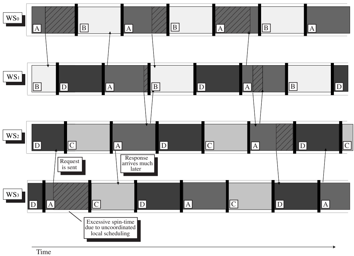
Figure 3.1: Local Scheduling. Four communicating jobs (A, B, C, and D) are allocated to four workstations. If the processes composing those jobs are scheduled by independent operating system schedulers on each workstation, then the communicating processes are not scheduled simultaneously across workstations. As a result, if a process spin-waits after sending a reply message until the reply arrives, CPU time will not be used effectively.
