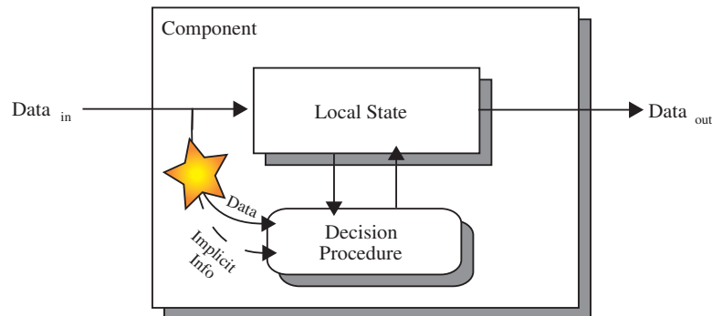
Figure 2.1: Model of an Implicitly-Controlled System. Components that are implicitly-controlled do not receive explicit control messages from other components in the system. Instead, components infer control information from naturally-occurring data transfers.
