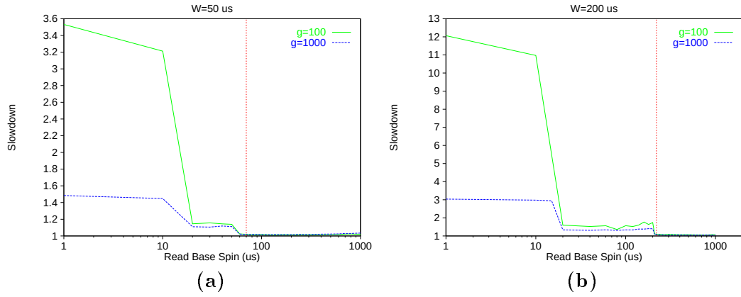
Figure 8.5: Sensitivity to Read Baseline Spin for Bulk-Synchronous Programs. The workload consists of three bulk-synchronous jobs on 32 workstations. The two lines designate different synchronization granularity; the time between barriers, g , is set to either 100 \mu s or 1 ms . The vertical line in each graph designates the desired read baseline spin, S_{Base}^R = 2L + W . There is no load-imbalance ( V = 0 ), and the time between reads after the barrier is fixed at c = 8 \mu s . The metric along the y-axis is the slowdown of the workload when implicitly coscheduled with two-phase waiting versus explicit coscheduling with spin-waiting. Along the x-axis, the baseline spin for reads is varied between 1 \mu s and 1000 \mu s , while the baseline spin for barriers is fixed at S_{Base}^B . When a process wakes after a message arrival other than the desired message, it spins for S_{Wake} = W . Network latency is fixed at L = 10 \mu s . In Figure a, the context-switch time is set to W = 50 \mu s ; in Figure b, W = 200 \mu s . Note the change in scale along the y-axes across the two graphs.
