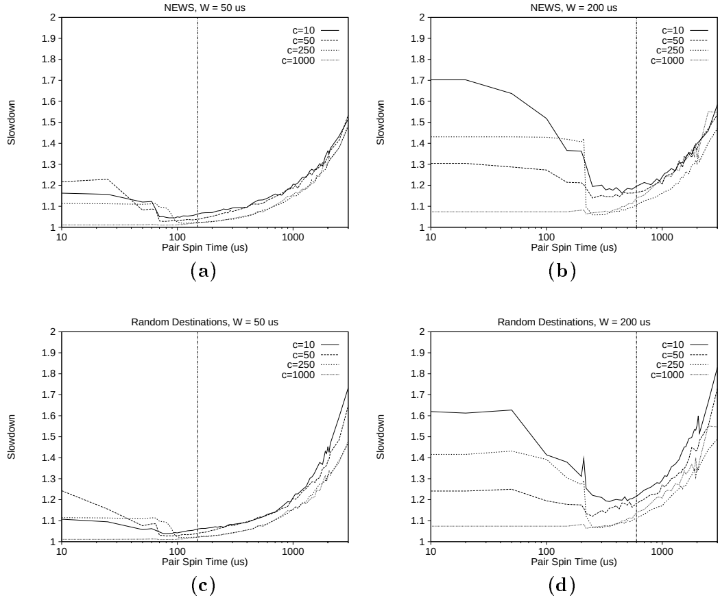
Figure 8.11: Sensitivity to Conditional Spin for Continuous-Communication Programs with Frequent Barriers. The experimental setup is identical to that in the preceding figures, except the time between barriers is set to g = 1ms instead of g = 100ms . Again, the vertical line marks 3W , our chosen value of S_{Cond}^R . Note that the point c = 2ms is not shown because it is not possible for c > g in this workload.
