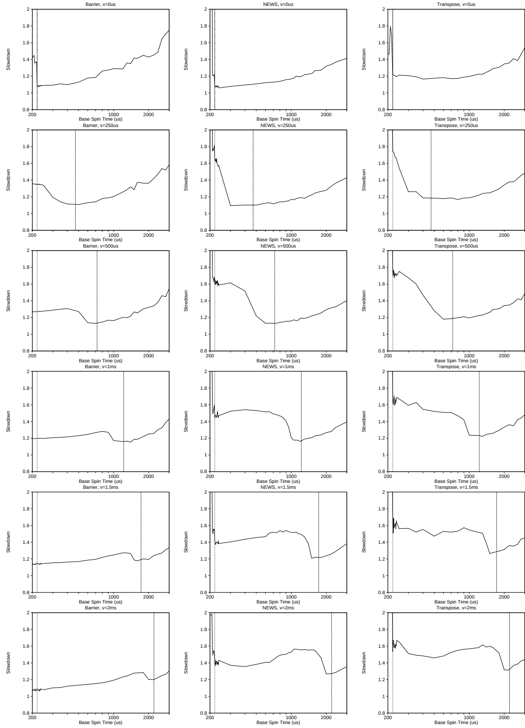
Figure 8.13: Sensitivity to Baseline Spin for Bulk-Synchronous Programs with Load-Imbalance ( W = 200\mu s ).
