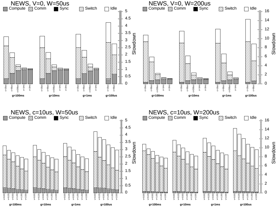
Figure 8.4: Performance of Immediate Blocking for Continuous-Communication Programs. The graphs show the slowdown of uncoordinated scheduling with immediate blocking versus explicit coscheduling for the NEWS communication pattern and two context-switch costs, W = 50\mu s and W = 200\mu s . In the top two graphs, load-imbalance is fixed at V = 0 ; along the x axis, the time between barriers, g , and the time between reads, c , are both varied. In the bottom two graphs, c is fixed 10\mu s and g and V are varied. In all graphs, network latency is set to L = 10\mu s .
