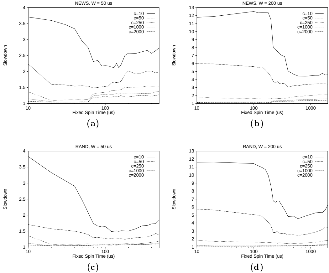
Figure 8.7: Sensitivity to Baseline Spin for Continuous-Communication Programs. Three continuously communicating applications are time-shared on 32 workstations. The time between barriers is set to g = 100\text{ms} with no load-imbalance ( V = 0 ). Each line in the graphs designates a different communication granularity, c . The metric along the y-axis is the slowdown of the workload when implicitly coscheduled with two-phase waiting versus explicit coscheduling with spin-waiting. Along the x-axis, the baseline spin amounts for both reads and barriers are changed simultaneously. In Figures a and c, the context-switch cost is set to W = 50\mu\text{s} ; in Figures b and d, W = 200\mu\text{s} ; note the change in scale along the y-axis between the two sets. In the top two graphs, processes communicate in a repeated NEWS pattern; in the bottom two graphs, processes communicate with random destinations.
