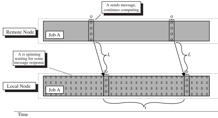
Figure 6.7: Cost of Incoming One-Way Requests if Local Process Spin-Waits. To help calculate T_{Cond}^O , this figure illustrates the cost to the local (receiving) process when it spin-waits between message arrivals. We assume a constant time t between message arrivals.
