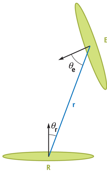
Figure 14-3. The Relationship Between Receiver and Emitter Elements
