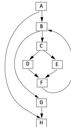
Control Flow Graph
