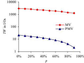
Figure 11. TW for transaction T .
