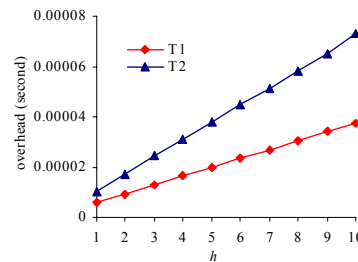
Figure 9. Overhead of our techniques (combination factor experiment).
