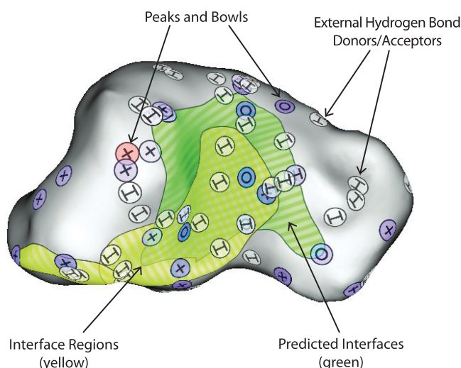
Figure 4. Stickers: four types of stickers are applied to abstracted surfaces, each of which may be independently turned on or off. 'Hydrogen bond stickers' are placed on the surface in areas that are close to one or more atoms that could form an external hydrogen bond. 'Detected Pocket stickers' indicate regions of the surface that resemble binding pockets, according to a variant of the LIGSITE pocket detector. 'Interface stickers' indicate regions of the surface in close proximity to another chain. And 'peak/bowl stickers' display as an 'X' or 'O', respectively, points where significant peaks or bumps in the original solvent excluded surface were removed.
