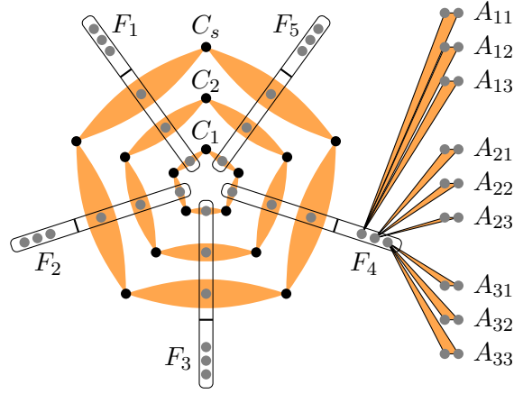
Figure 2: A coordination gadget as in Lemma 3.1 for d = 3 , s = 3 and m = 2 . All vertices are drawn, and all edges of the odd cycles C_i . The boxes for the F_j represent even cycle gadgets from Figure 1. All edges between the A_{k,\ell} and F_4 are drawn, but all other edges incident to the A_{k,\ell} are omitted. They attach to the other F_j in a similar fashion.
