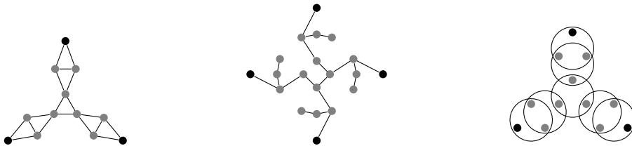
Figure 3: Hyperedge gadgets for different H -matching problems. The outermost, black vertices are the vertices of the simulated hyperedge and the gray vertices are not supposed to be adjacent to any other vertex of the graph. Left: Triangle matching. Middle: 3-Path matching. Right: The general case; each circle represents a copy of H .
