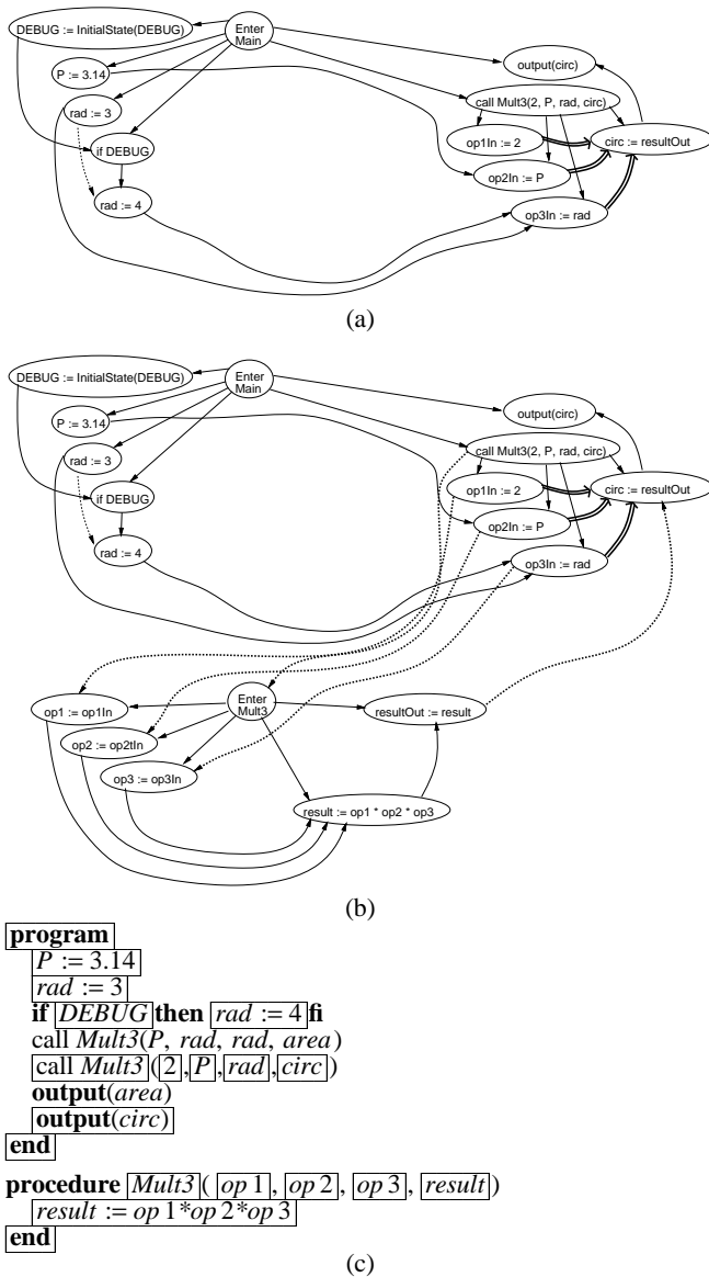
Figure 7. A backward (interprocedural) slice of the SDG of Figure 3 with respect to component “ output(circ) ”. The vertices reached during Pass 1 as well as their induced edges are shown in (a); the vertices and edges added by Pass 2 are shown in (b); the components of the program that correspond to the vertices identified by the slice are shown in (c).
