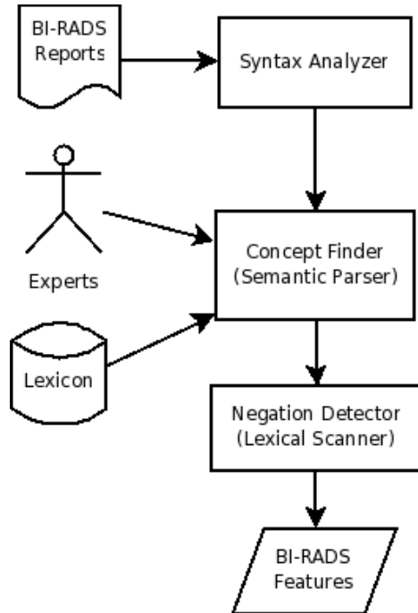
Fig. 2. Algorithm flowchart
