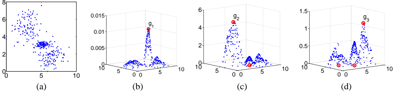
Figure 1: (a) A toy data set. (b) The stationary distribution \pi reflects centrality. The item with the largest probability is selected as the first item g_1 . (c) The expected number of visits v to each node after g_1 becomes an absorbing state. (d) After both g_1 and g_2 become absorbing states. Note the diversity in g_1, g_2, g_3 as they come from different groups.
