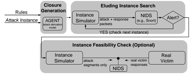
Figure 2. AGENT Architecture.
