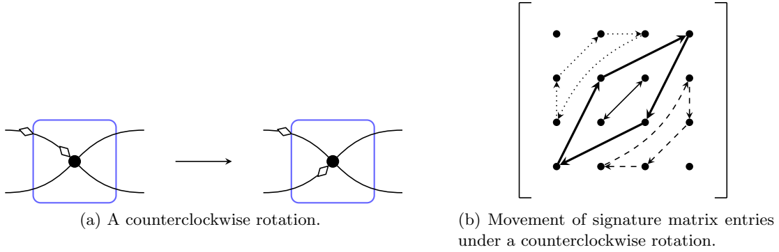
Figure 4: The movement of the entries in the signature matrix of an arity 4 signature under a counterclockwise rotation of the input edges. The Hamming weight one entries are in the dotted cycle, the Hamming weight two entries are in the two solid cycles (one has length 4 and the other one is a swap), and the entries of Hamming weight three are in the dashed cycle.
