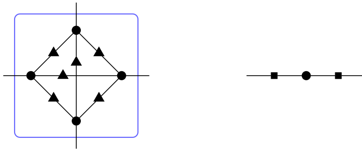
(a) The tetrahedron gadget with edge signatures given in (b).
