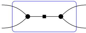
Figure 9: The circles are assigned [t, 1, 0, 0] and the square (\neq_2) .
