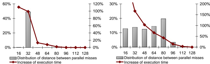
Fig. 1. Comparison of the distribution of distances between parallel L2 misses and performance degradation due to IQ resizing for gcc and art
