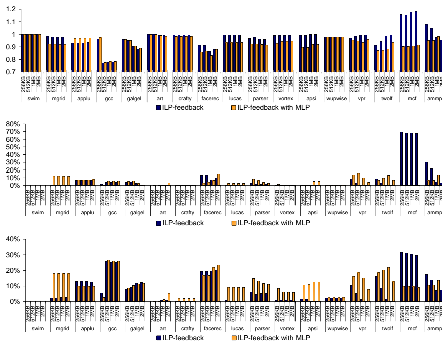
Fig. 5. Normalized Energy-Delay Product (a), Execution Time Increase (b) and Energy Savings (c) for best configurations: ILP-Feedback (256 threshold) and ILP-Feedback with MLP (512 threshold)
