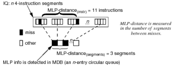
Fig. 3. MLP Distance Buffer (MDB): A circular queue keeps aggregate information corresponding to IQ segments
