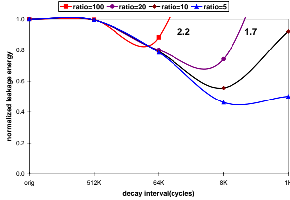
Fig. 18. Normalized L1 data cache leakage energy for cache decay methods on a multiprogrammed workload.
