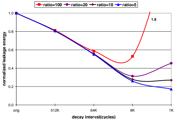
Fig. 9. Normalized L1 data cache leakage energy averaged across SPEC suite for various L2Access:leak ratios.
