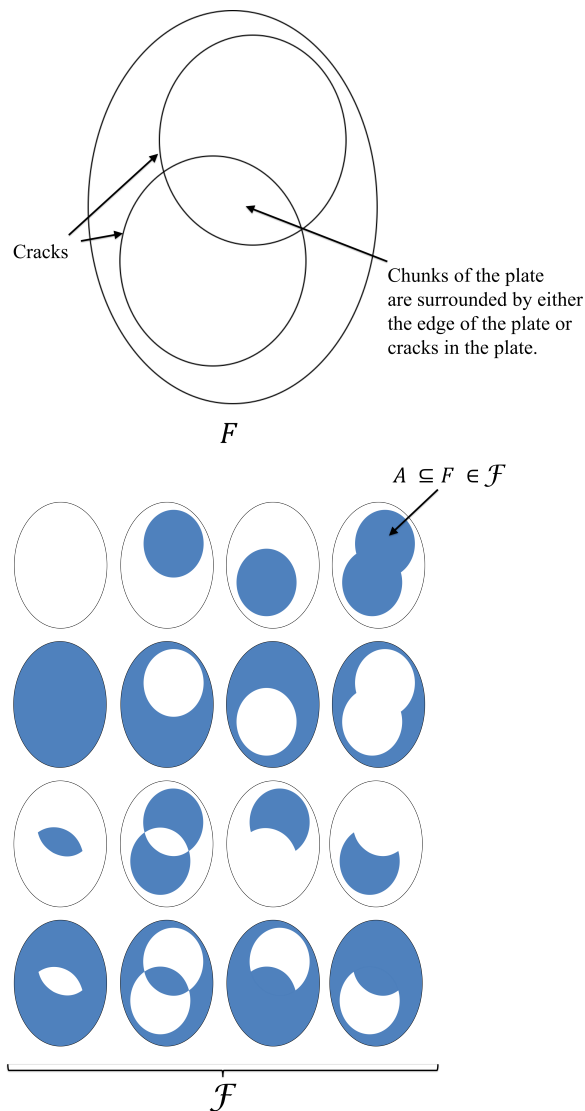
Figure 1: The large oval above is a ceramic plate with cracks along its surface. Let the points on the plate be a set F . Below, we illustrate every subset A \subseteq F where A represents the plate with some combination of chunks of the plate removed. We are only allowed to remove a chunk if it is surrounded by cracks. The entire set of configurations of ways we can removing chunks of the plate is a \sigma -algebra \mathcal{F} over F .
