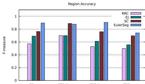
Figure 9: F-measure scores on datasets described in Section 5.
