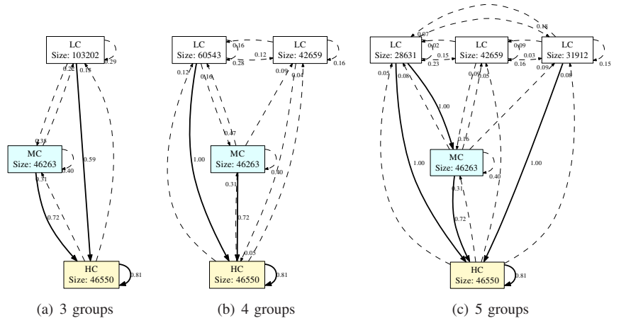
Fig. 3. Graph summaries for the CiteSeer dataset
