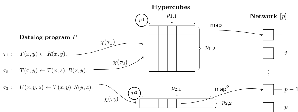
■ Figure 2 Example of a GHP policy for the Datalog program P with three rules.
