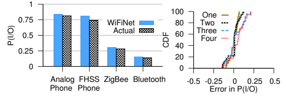
Figure 9: Accurately identifying impact of each interferer in the presence of multiple non-WiFi devices. (left) example scenario showing WiFiNet is able to identify the strong interferers (analog cordless phone, FHSS phone) and weak interferers (ZigBee and Bluetooth devices) accurately. (right) CDF of error in inference estimates in the presence of multiple interferers.
