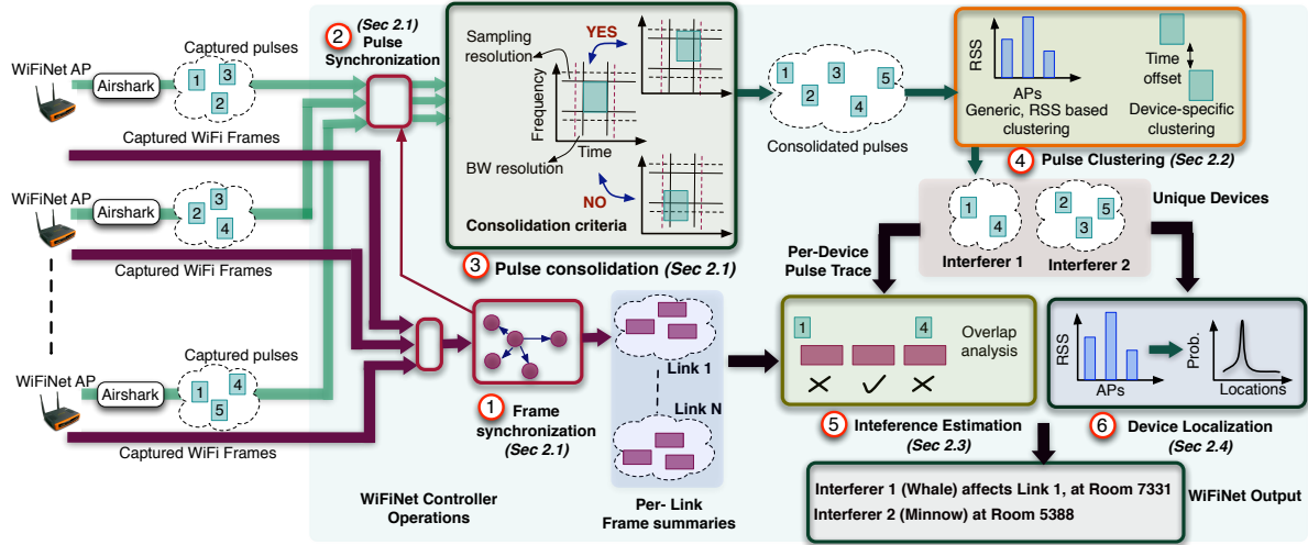
Figure 2: Flow of operations in Wi-FiNet. Wi-FiNet APs capture spectral samples as well as WiFi frames. Each AP runs Airshark [16] to detect non-WiFi devices and output non-WiFi pulses (transmissions) tagged with device type. (1) WiFi frames are used to synchronize the clocks at the APs. (2,3) Synchronized clocks at the APs are then used to consolidate the pulses across multiple APs using a heuristic (§2.1). (4) Consolidated pulses are clustered using RSS and device-specific attributes to output unique non-WiFi device instances and their pulses (§2.2). (5) For each non-WiFi device instance and WiFi link, the interference estimation module analyzes the impact of the device on the link using transmission overlaps (§2.3). (6) Model-based localization algorithms are used to localize each non-WiFi device instance (§2.4).
