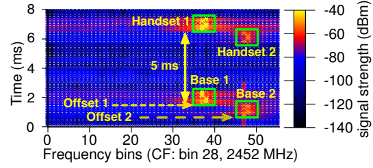
Figure 3: Heatmap of 4 FHSS cordless phone devices (2 base/handset pairs) captured by a WiFiNet AP showing the timing property.
