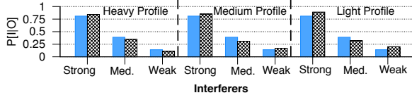
Figure 14: WiFi links replay real HTTP/TCP wireless traces [17] (heavy, medium, and light profiles) in presence of strong, medium and weak interferers. WiFiNet’s estimates closely match the ground truth in each case. The slight mismatch is due to the variability in packet sizes as the ground truth was measured using 1400 byte packets, whereas the traces comprised packets of different sizes.
