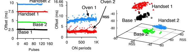
Figure 4: Segregating pulses in the presence of multiple, simultaneously operating devices of the same type, based on WiFiNet’s device specific and generic clustering. Figure shows clusters of pulses from (left) 2 FHSS cordless phone base/handset pairs (4 FHSS cordless devices) using pulse start time offset (middle) 2 Microwave ovens using ON-period offset (right) 4 FHSS cordless devices using a generic, RSS based k -means + EM-clustering technique using 3 WiFiNet APs.
