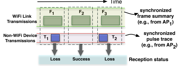
Figure 5: Illustration of interference estimation in WiFiNet.
