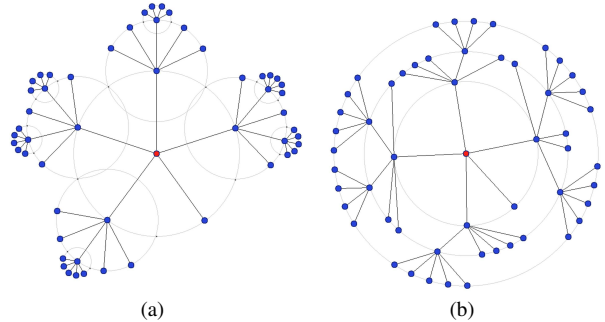
Figure 1: Two drawings for the same tree: Figure 1(a) is drawn by our layout algorithm, and Figure 1(b) is drawn by Yee et al.’s layout algorithm for Gnutellavision [26].
