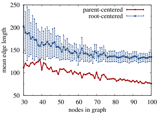
Figure 7: Spanning tree sibling edge lengths Edge lengths from siblings to their common parent tend to decrease as graph size increases. In our algorithms, siblings are positioned equidistant to their common parent. In Yee et al.’s algorithms, edge lengths from siblings to common parent vary, as shown by standard deviations.
