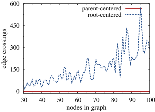
Figure 5: Isomorphic tree transitions Our parent-centered visualization scheme produces no edge crossings when transitioning between drawings of the same tree, while Yee et al.’s root-centered system produces many.
