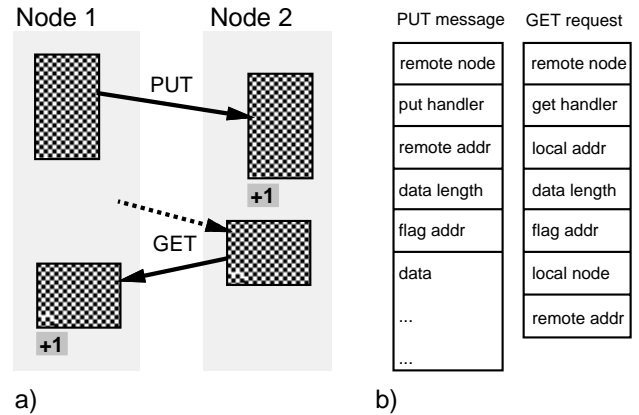
Figure 3: Split-C PUT and GET perform split-phase copies of memory blocks to/from remote nodes. Also shown are the message formats.
