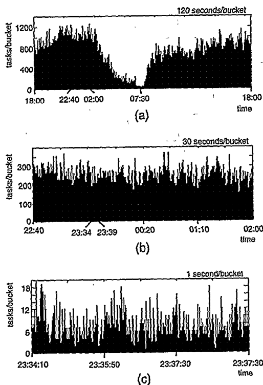
Figure 6: The number of requests per second for traced dialup IP users, showing burstiness across different time scales. (a) 24 hours with 2 minute buckets, 5.8 req/s avg., 12.6 req/s max. (b) 3 hr 20 min with 30 second buckets, 5.6 req/s avg., 10.3 req/s peak. (c) 3 min 20 sec, 8.1 req/s avg., 20 req/s peak.
