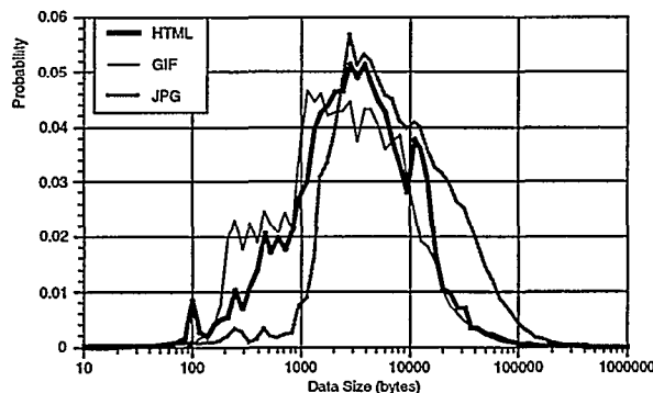
Figure 5: Distribution of content lengths for HTML, GIF, and JPEG files. The spikes to the left of the main GIF and JPEG distributions are error messages mistaken for image data, based on file name extension. Average content lengths: HTML - 5131 bytes, GIF - 3428 bytes, JPEG - 12070 bytes.
