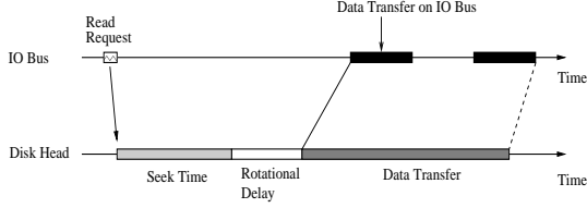
Figure 1: Timing diagram for a disk read request.
