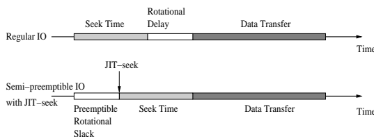
Figure 4: JIT-seek.
