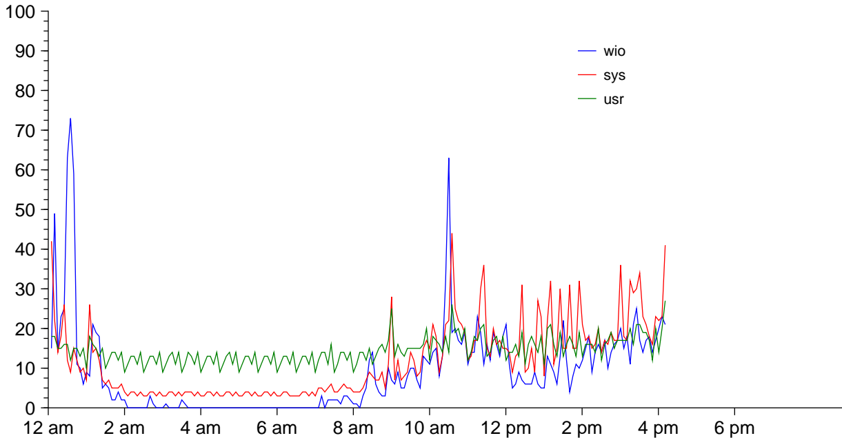
% CPU Utilization
