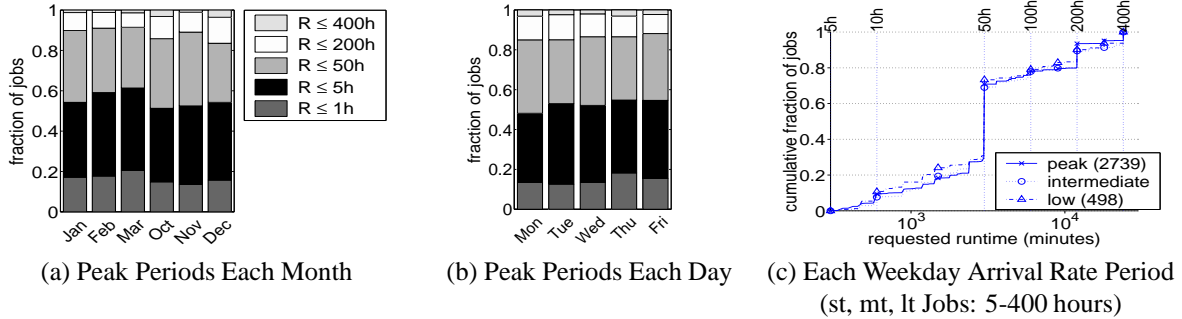
Figure 9. Variation in Distribution of Requested Runtime (R)
