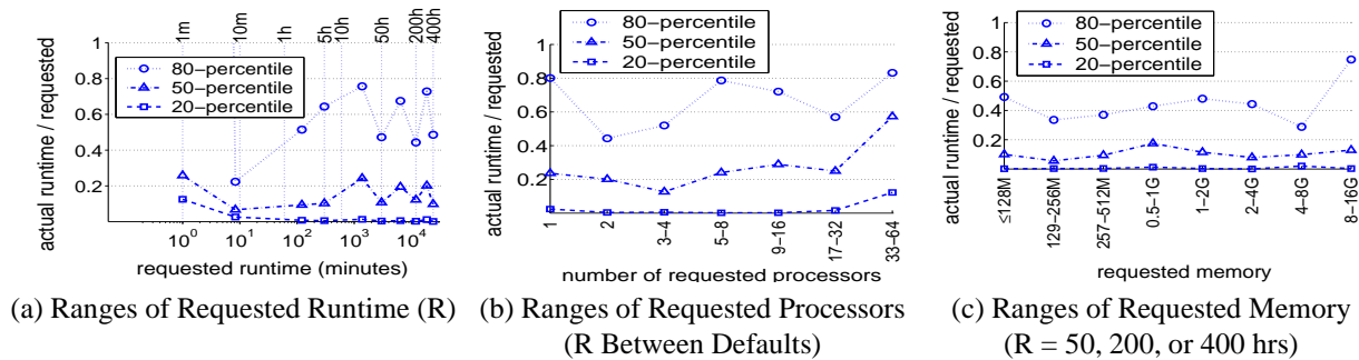
Figure 13. Actual Runtime/Requested Runtime For Various Resource Request Classes (October-December 2000)
