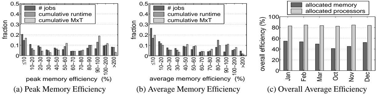
Figure 16. Memory Efficiency
