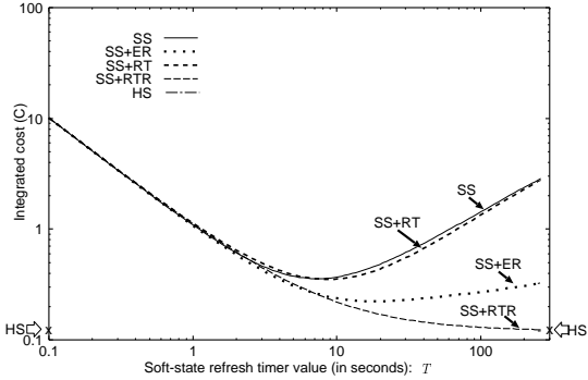
Figure 7: Soft-state refresh timer ( T )
