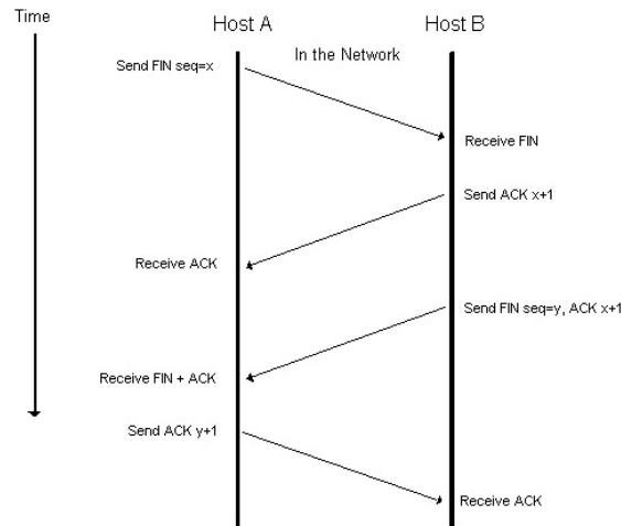
Figure 2: Three way handshake
