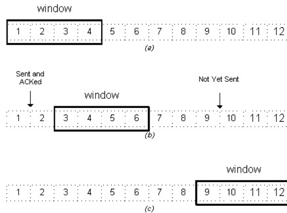
Figure 3: Sliding Window Protocol
