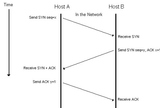
Figure 1: Three way handshake
