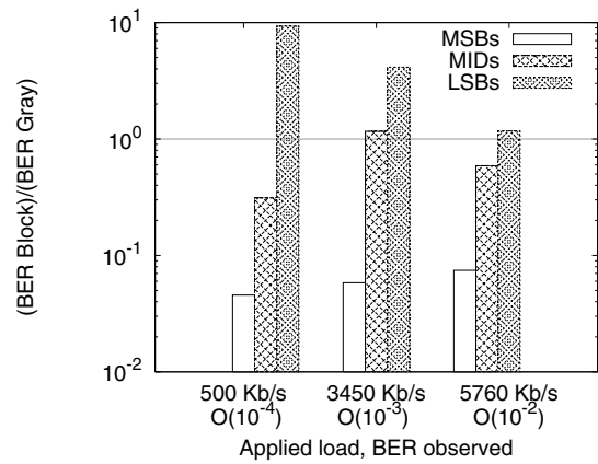
Figure 9: Variation in BER gain at various bit positions of Block relative to Gray in presence of an external interferer. Convolution coding at rate 1/2. The horizontal line corresponds to the case where both schemes offer equal error protection for a given bit position.
