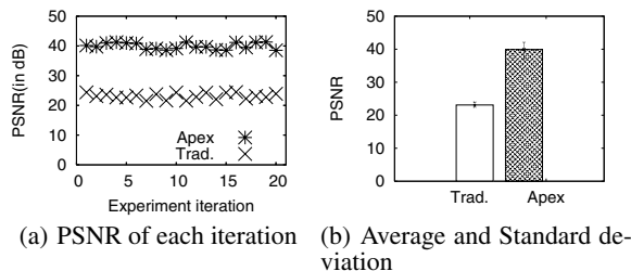
Figure 12: PSNR differences between traditional and approximate communication with rate adaptation at a representative wireless environment (Claire video).
