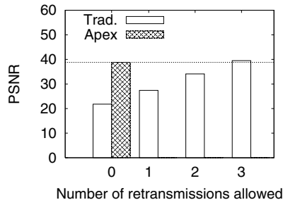
Figure 16: Variation in PSNR for traditional communication (with different number of retransmissions) and Apex (without retransmissions).
