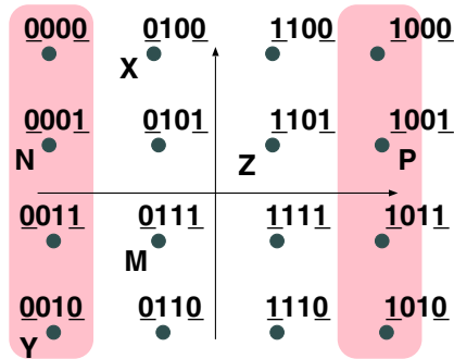
Figure 4: 16-QAM with Gray code constellation map. MSBs and LSBs are underlined.
