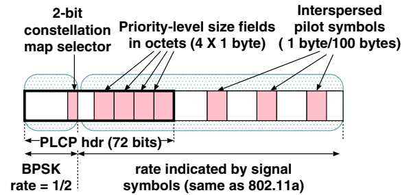
Figure 11: Modifications to PHY PLCP header and payload for Apex.
