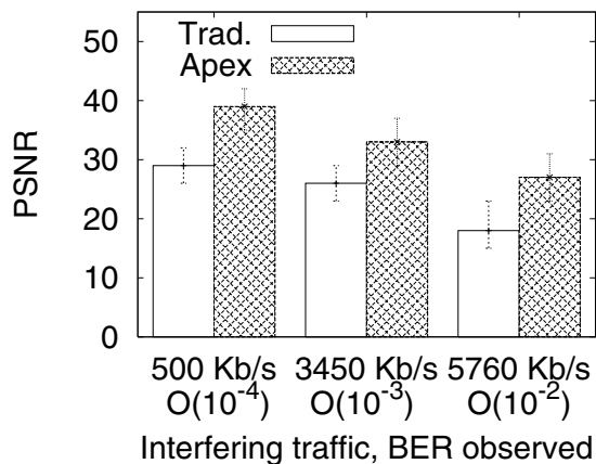
Figure 14: PSNR for traditional and approximate communication under varying external interference (Claire video). X-axis marks both the imposed (802.11) interference load on the channel and the corresponding average uncoded BER.
