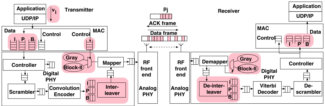
Figure 10: Changes to basic 802.11 layers for approximate communication in Apex. I, P, B labels are for illustration purpose only indicating three arbitrary priority layers. Shaded parts are modifications made.
