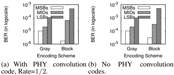
Figure 7: BER of various bit positions when using Gray, and Block data coding schemes. The overall uncoded BER of during the experiment was order of 10^{-3} for both schemes. 10 million QAM-64 symbols were transmitted.
