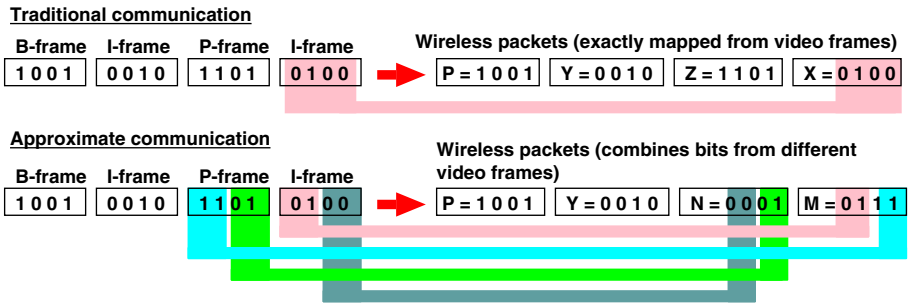
Figure 5: Wireless frames in approximate communication combines bits from video frames of different priority levels. Example uses 16-QAM and assumes that the two MSBs can be better protected than the two LSBs. The data bit placement strategy maps I-bits MSBs and P- and B-bits to LSBs. Symbols M , N , P , X , Y , and Z are as shown in Figure 4 that uses a Gray code constellation map. (Only subset of data bit placements shown.)
