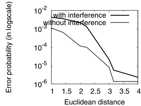
Figure 3: Fast decay in probability of erroneous decoding as the distance between the correct symbol and the erroneously decoded symbol increases. Data based on 10 million known 64-QAM symbols transmitted. In the ambient noise scenario, the overall BER was 3 \times 10^{-4} . In the explicit interference scenario, the overall BER was 6 \times 10^{-3} .
