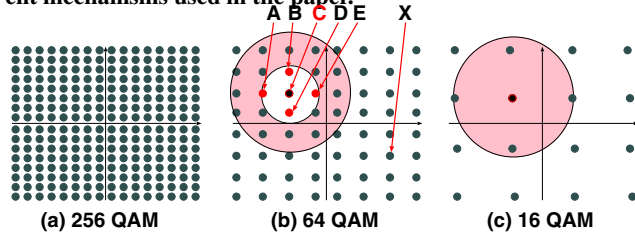
Figure 2: Quadrature Amplitude Modulation (QAM) constellations.
