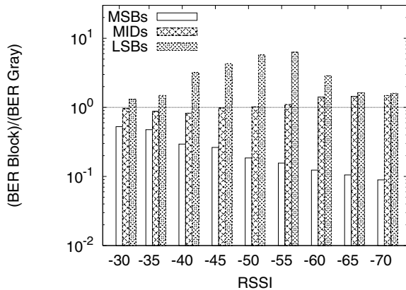
Figure 8: Variation in BER gains at different bit-positions with Block relative to Gray with varying RSSI, and with PHY convolution coding at rate 1/2. The horizontal line corresponds to the case where both schemes offer equal error protection for a given bit position.
