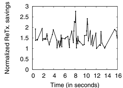
Figure 17: Saved retransmissions in Apex. Y-axis shows the normalized number of bytes transmitted by traditional communication (3 retransmissions) with respect to Apex.
