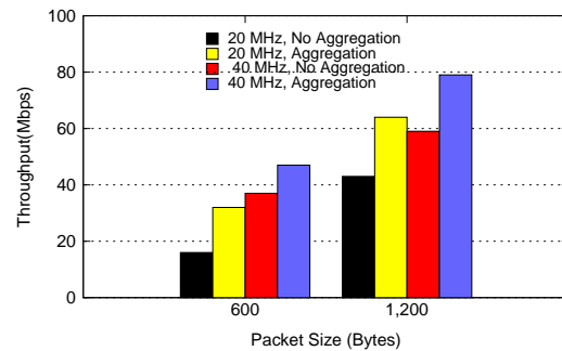
Figure 3: Average throughput achieved on an isolated 802.11n link under different combinations of channel width and aggregation mechanisms.
