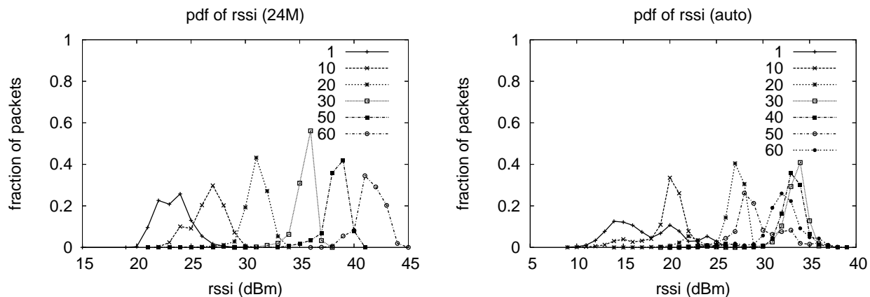
(a) Pdf of RSSI values on 802.11a (no interference). 6 distinct power levels can be observed (b) Pdf of RSSI values on 802.11g (interference with department WLAN). 4 distinct power levels can be observed
