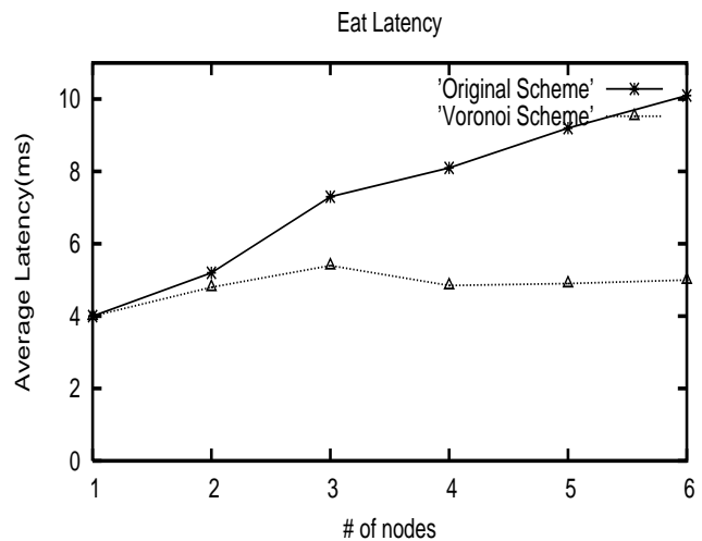
Fig7. Eat Latency as a function of Number of Players
