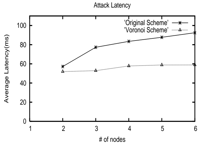
Fig. 6 Attack Latency as a function of Number of Players
