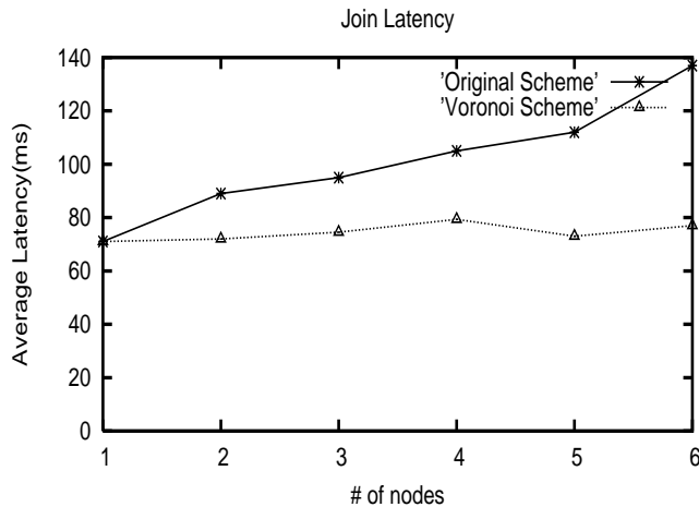
Fig5. Join Latency as a function of Number of Players
