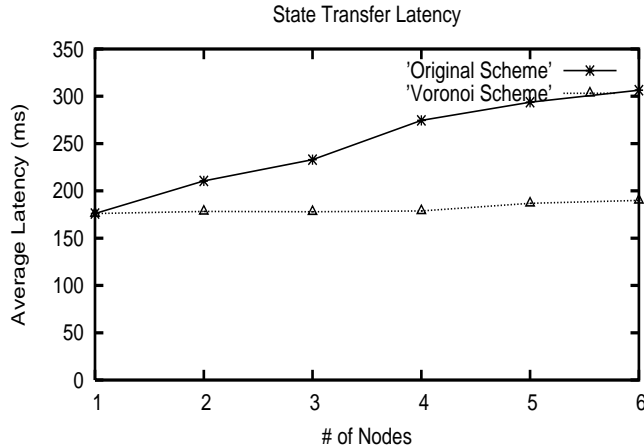
Fig.8 State Transfer Latency as a function of Number of Players Again, as seen from the graph, our implementation gives near constant performance. No single node has to handle the transfer between players. Each player maintains and exchanges almost constant amount of state.
