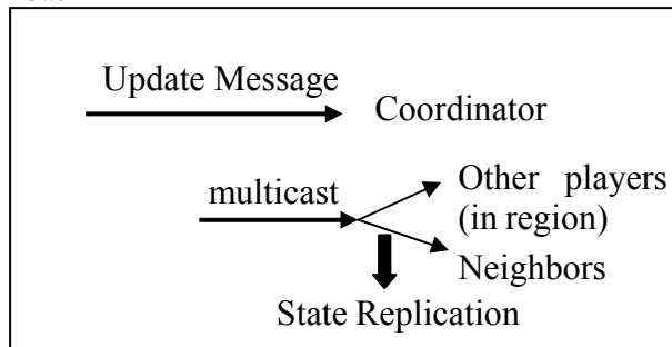
Fig 3. Message Flow in the System
