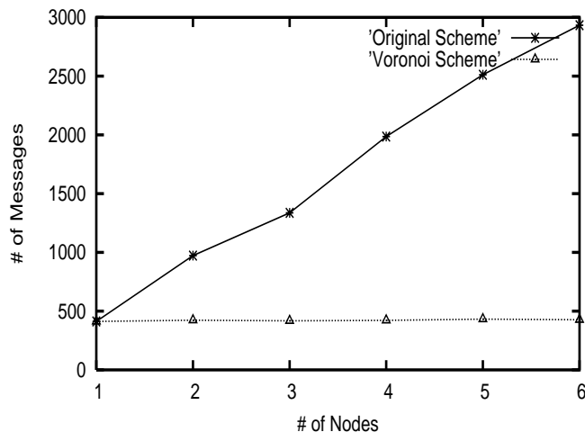
Fig 9. Number of Messages Sent and Received as a function of Number of Players
