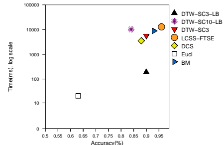
Fig. 13. Results of Surveillance classification by nearest neighbor using data from [36].
