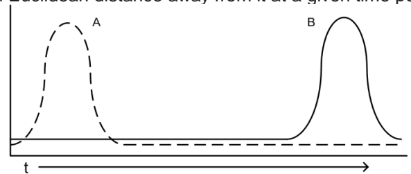
Fig. 4. The \delta factor is used to control dictionary segments from being improperly used. Here, segments that are produced by the peak of time-series A could be used during the compression of the peak of target series B. Further, both time-series have flat intermediary regions that are within small \epsilon . The compression sizes would be quite similar and erroneously give favorable similarity.
