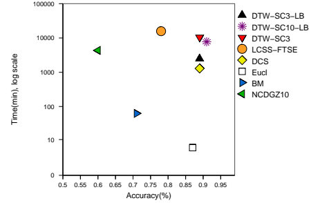
Fig. 12. Results of synthetic lightning (RS) classification by nearest neighbor using data from [23].
