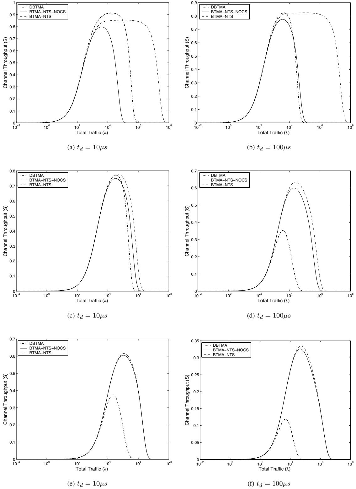
Fig. 3. Channel throughput comparison. \delta=4096 bits, \gamma=256 bits; in (a) and (b), channel data rate R=1 Mbps, radio range L=35 m; in (c) and (d) channel data rate R=10 Mbps, radio range L=1000 m; in (e) and (f) channel data rate R=50 Mbps, radio range L=1000 m.
