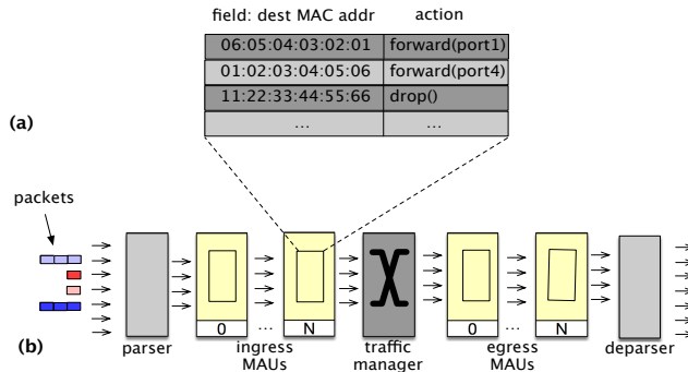
Figure 1: (a) A match-action table programmed to forward or to drop a packet according to its destination MAC address. (b) Architecture of a programmable switch dataplane holding that table.
