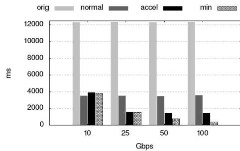
Figure 8: Effects of varying the network speed on four plans for TPC-H Query 20. Accelerated plans respond better to speed increases.
