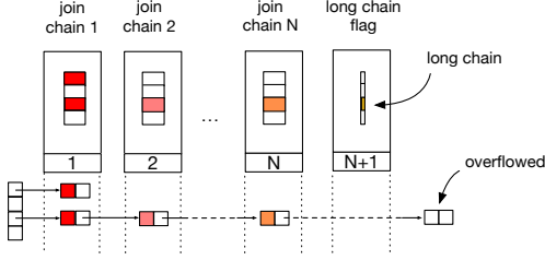
Figure 4: Stage layout for a hash table based on fixed-sized collision chain. The k -th stage, 1 \leq k \leq N , keeps track of the keys in the k -th position of every collision chain. An extra stage flags the collision chains having more elements than stages. Elements that do not fit are handled in the overflow area.
