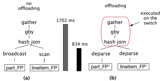
Figure 7: The (a) normal and (b) accelerated plans for the first join/group-by pattern of TPC-H Query 20. The bars indicate response times.
