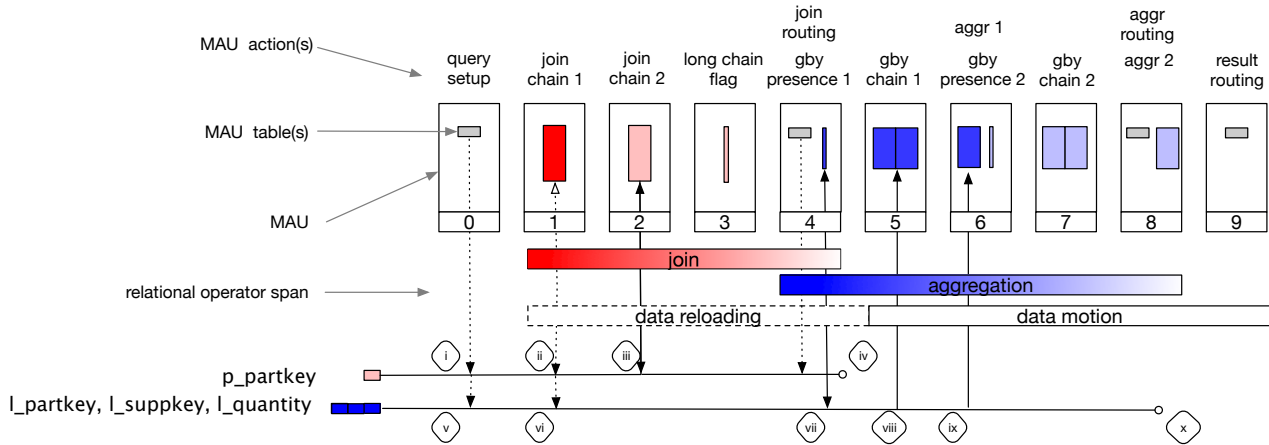
Figure 6: The join/group-by/reshuffle logic, as compiled from P4 sources, takes 10 MAUs. We are using hash-tables with fixed collision chains of two elements for both the join and the group-by. (Single column for the join and double for the group by.) Incoming tuples from the MPP nodes are processed at (i) and (v) where a tuple’s join and group-by hash indices are computed. The outer relation tuple (in red) reads the first entry in the collision chain (ii). That entry is occupied, so the tuple moves on to the next stage and gets inserted as a collision (iii). The tuple then gets marked to be dropped in (iv). The inner relation tuple (in blue) first probes the join hash-table. It matches a key in the first entry of the collision chain (vi) and so is allowed to proceed down the pipeline. In (vii), it identifies that its corresponding group-by table index is empty. It sets a bitmap to indicate it will take the position and gets inserted into the group-by hash table in (viii). It moves to the next stage where the initial aggregation value for that group is recorded (ix) before the tuple is marked to be dropped at (x).
