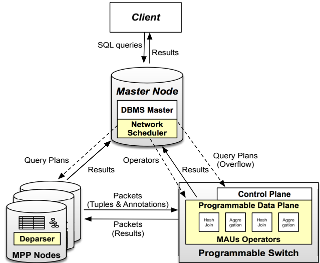
Figure 3: NETACCEL’s high-level architecture.
