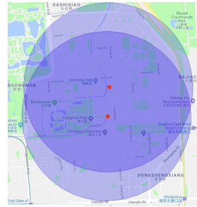
Figure 13. LoRa Gateway Locations in Tsinghua University
