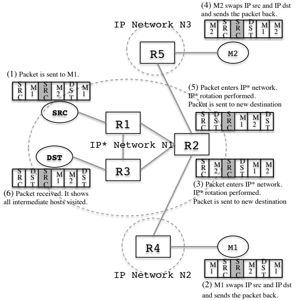
Figure 11: Example of an IP* network where a packet sent from SRC to DST visits middleboxes M1 and M2 . The figure labels 6 steps of packet processing along with the transformed header at each step. R2 is the entry point to the IP* network which performs IP* header updates.
